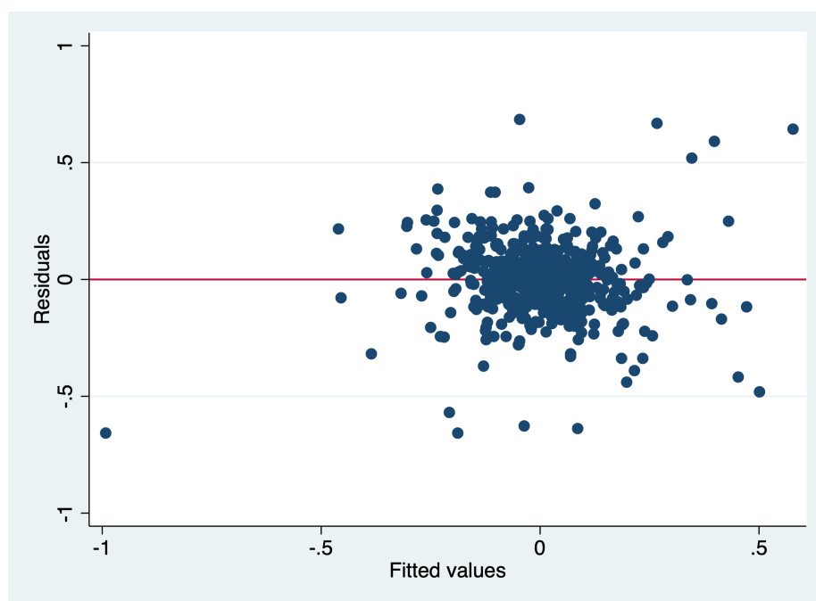
Figure 2.4: Plotting Errors
