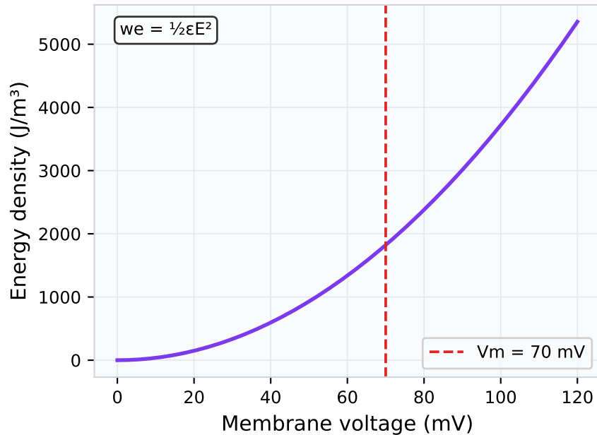
Stored Energy Density
