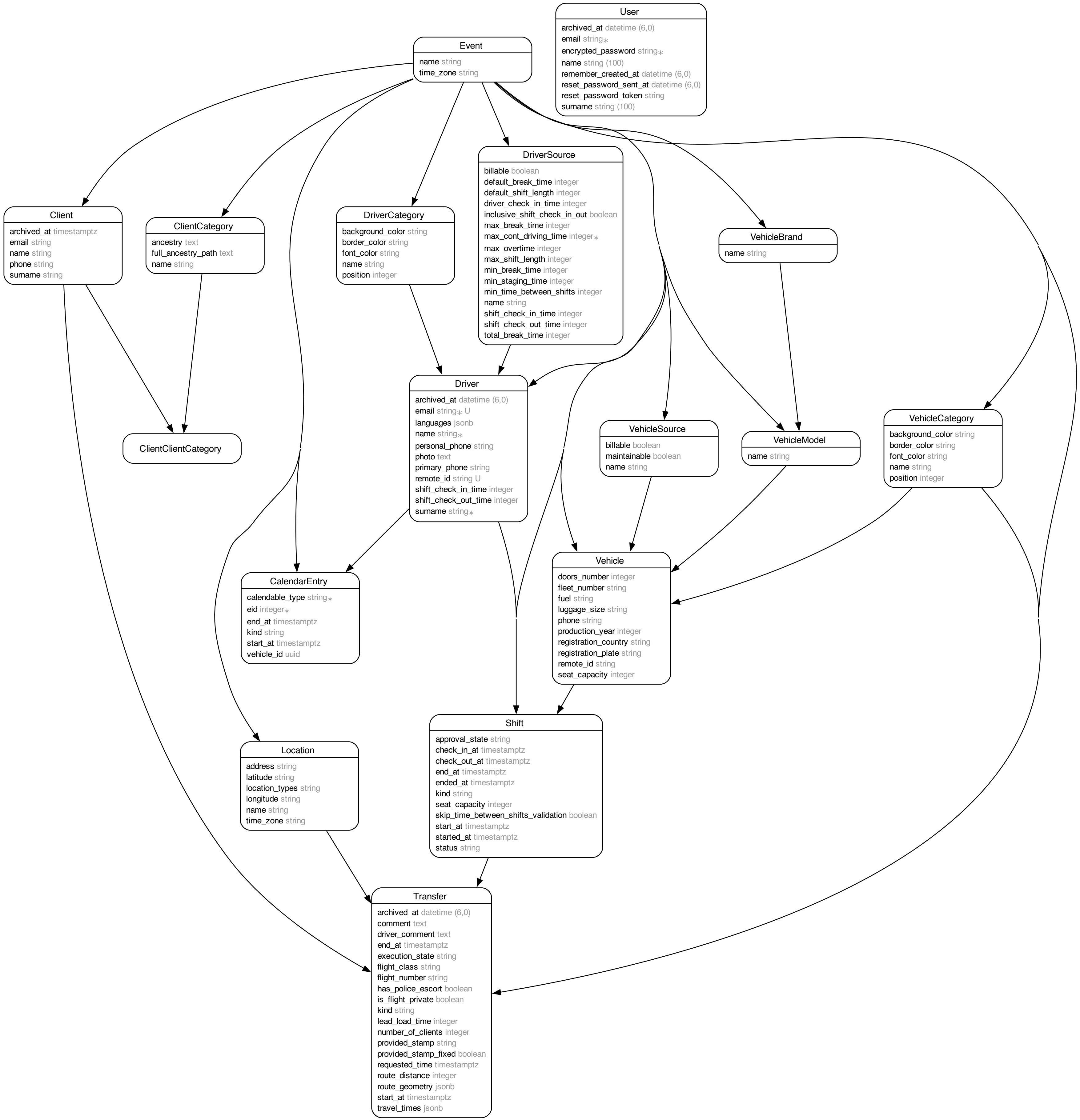
RecruitmentChallenge domain model
