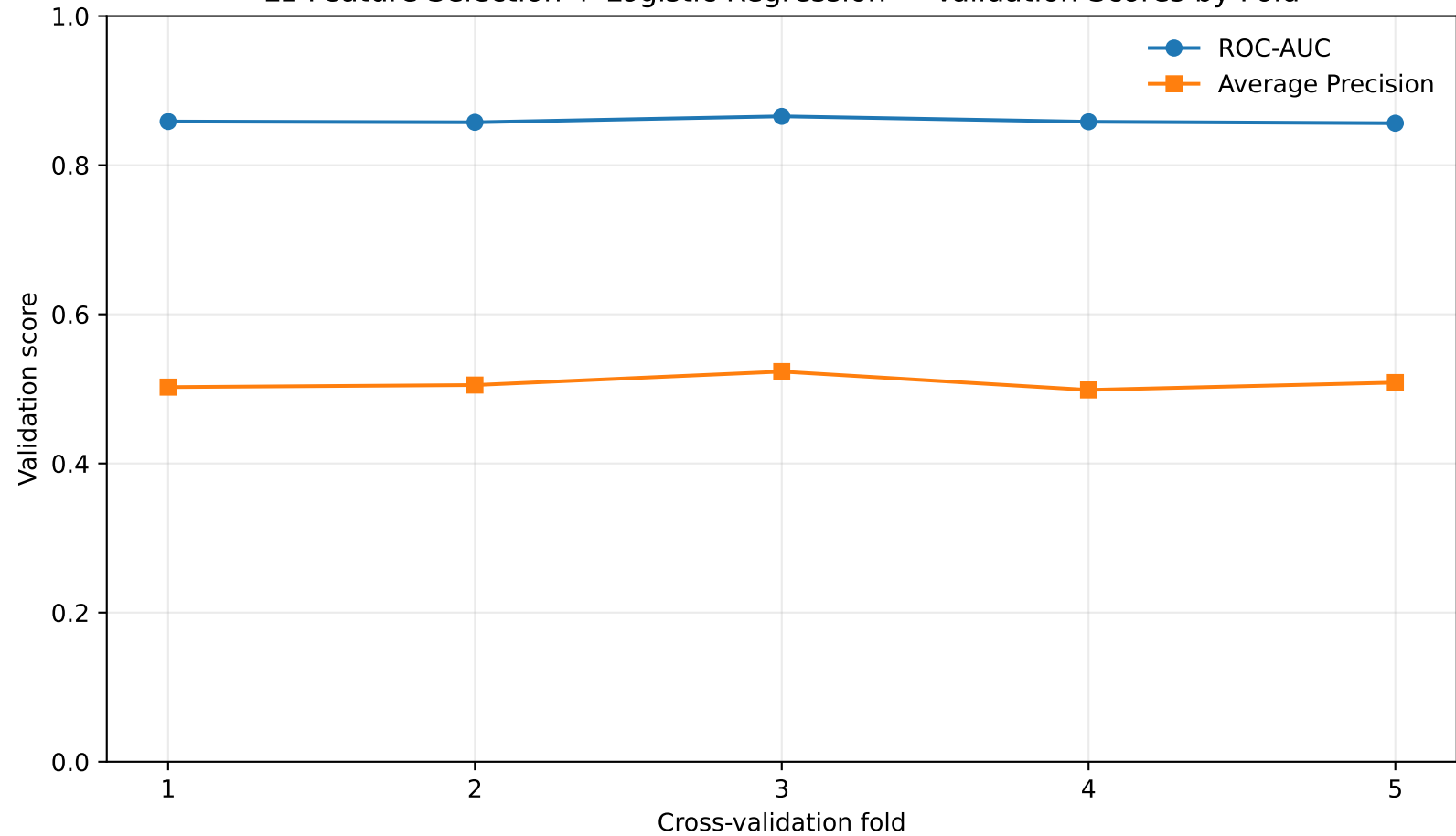
L1 Feature Selection + Logistic Regression — Validation Scores by Fold
