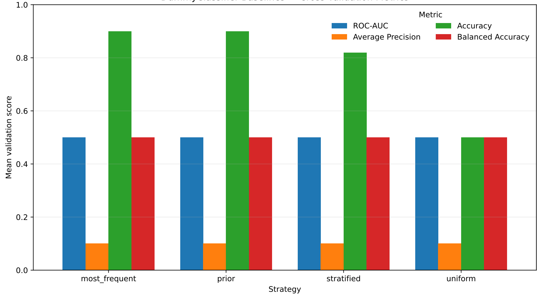
DummyClassifier Baselines — Cross-Validation Metrics
