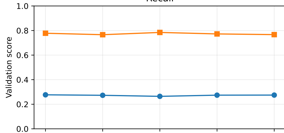
Recall
