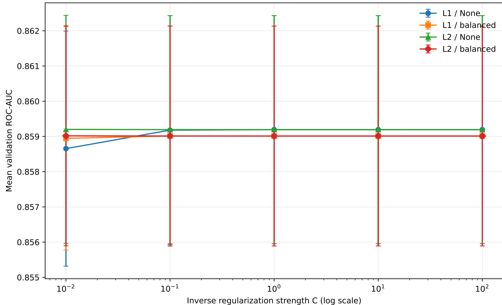
Logistic Grid Search — Validation ROC-AUC
