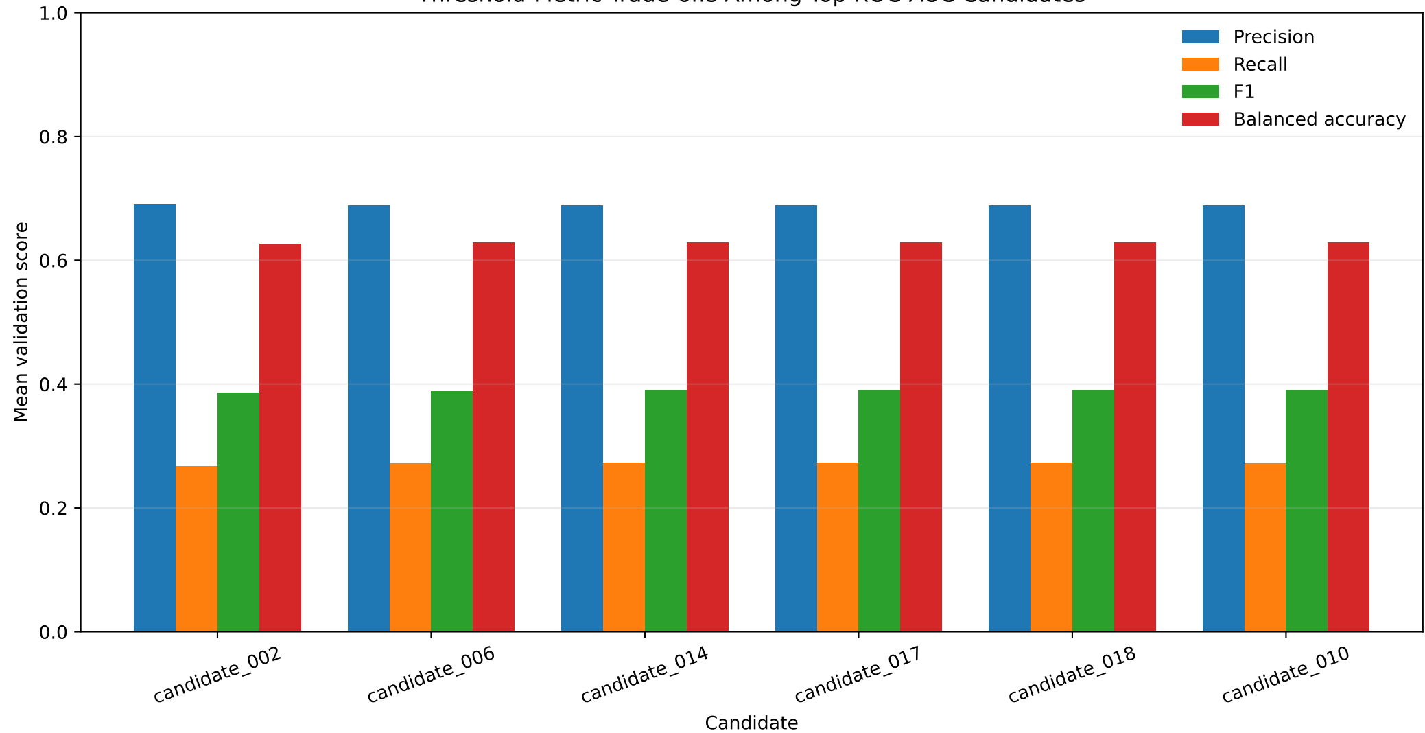
Threshold-Metric Trade-offs Among Top ROC-AUC Candidates
