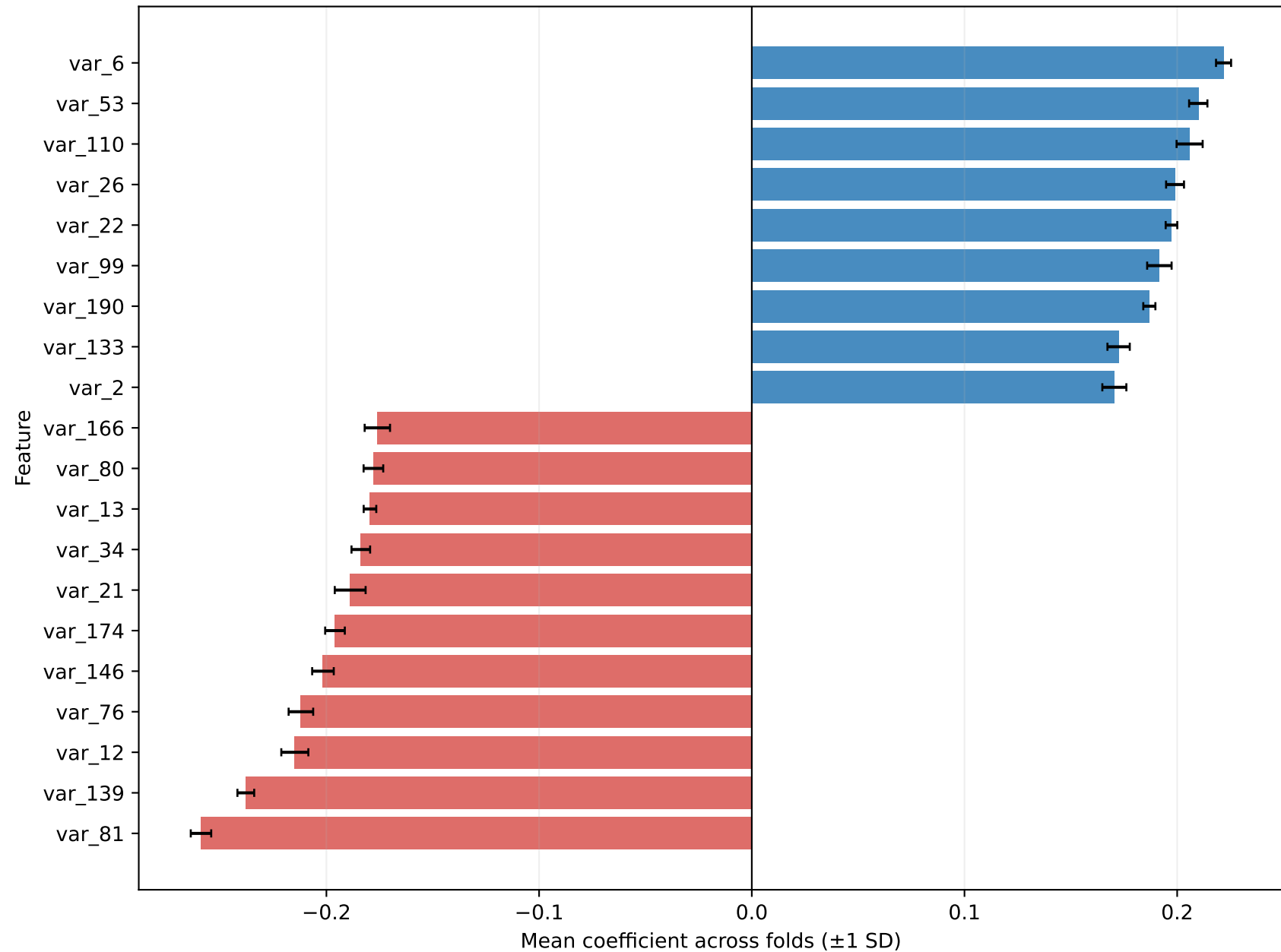
Top 20 Standardized Logistic Coefficients — LR-SELECTED-ROC
