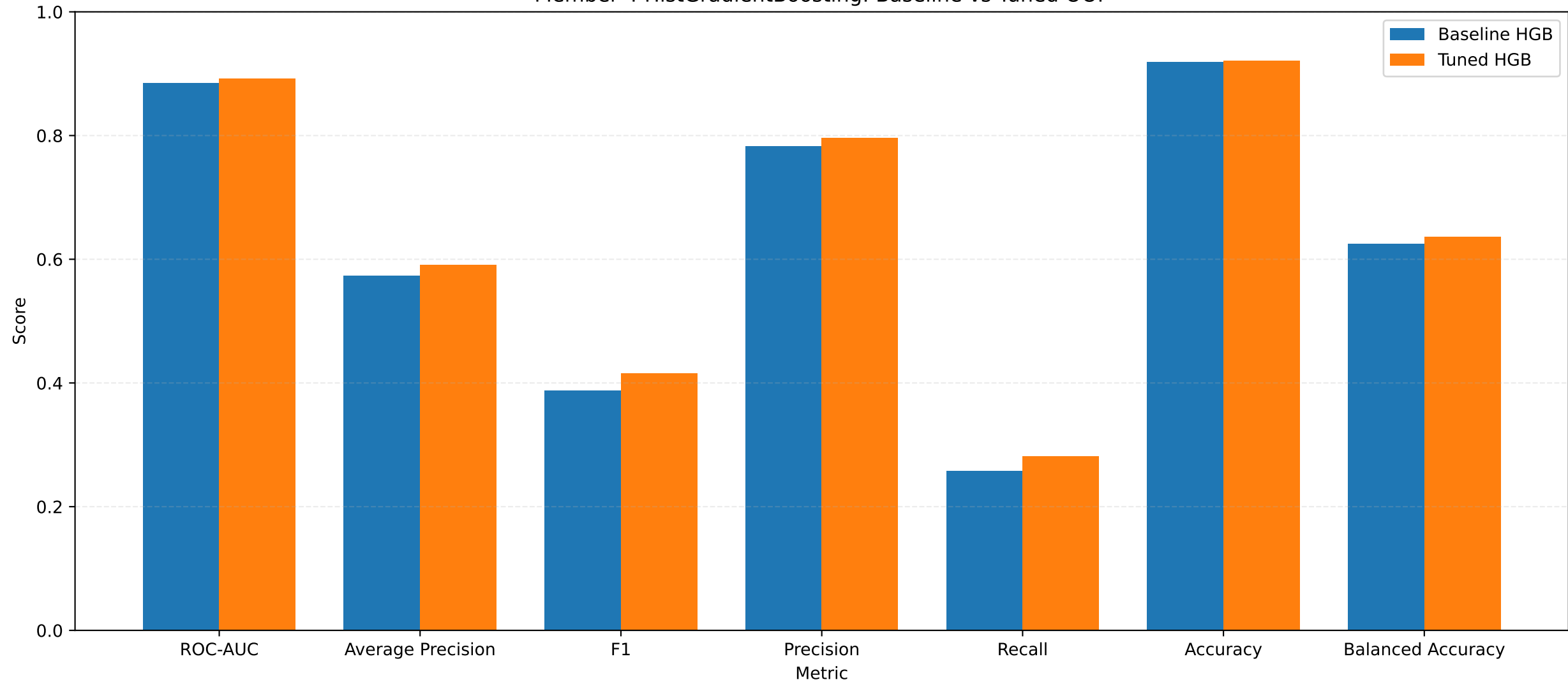
Member 4 HistGradientBoosting: Baseline vs Tuned OOF
