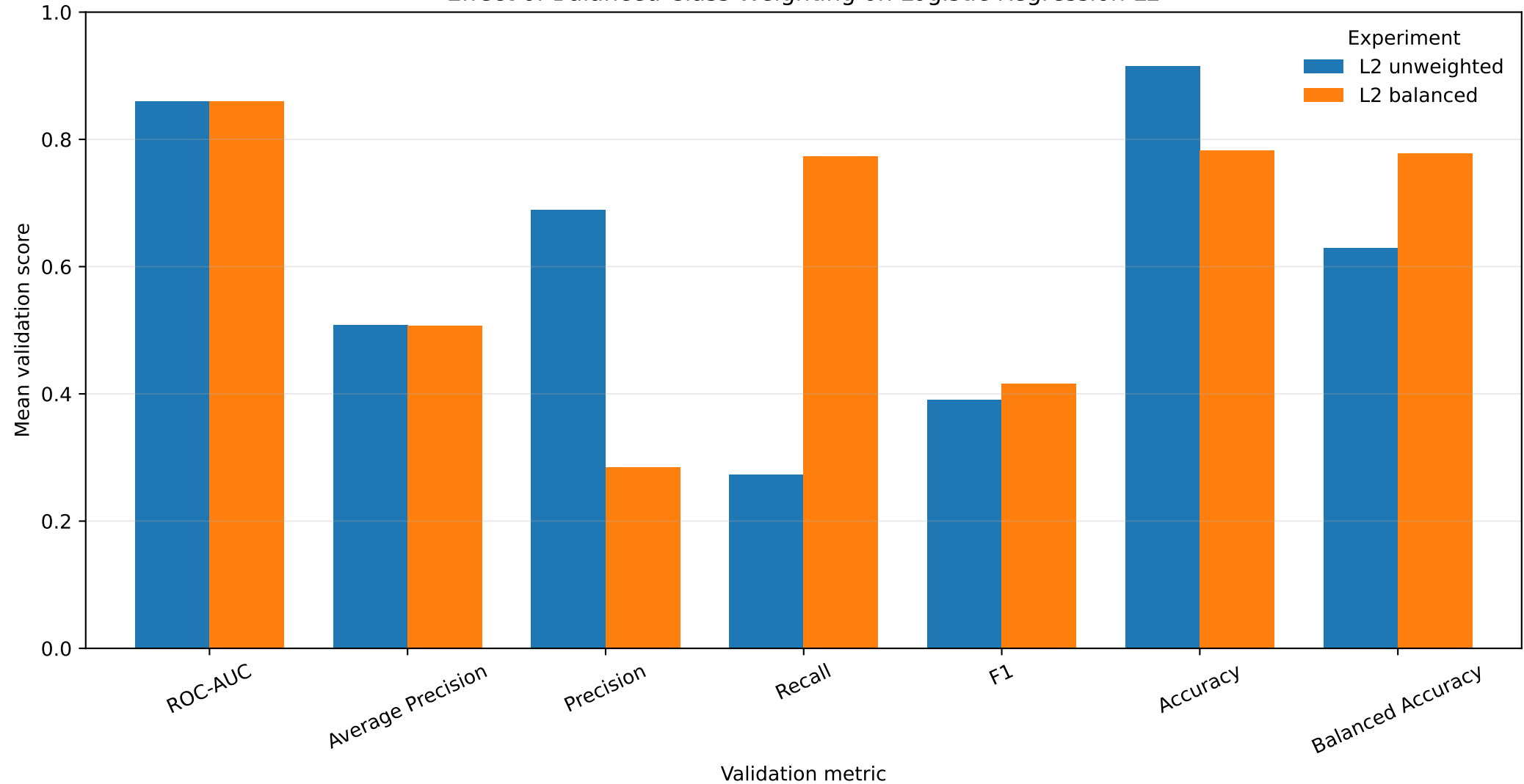
Effect of Balanced Class Weighting on Logistic Regression L2
