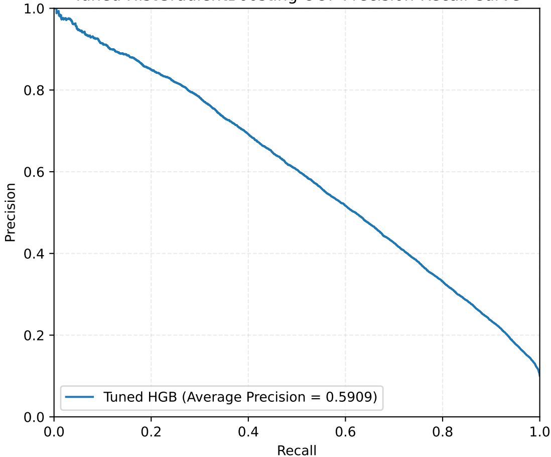
Tuned HistGradientBoosting OOF Precision-Recall Curve
