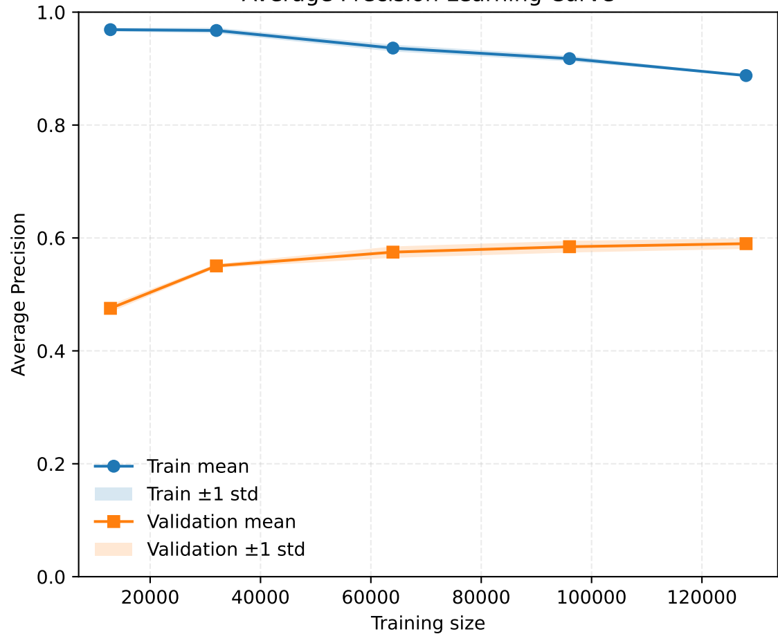
Average Precision Learning Curve
