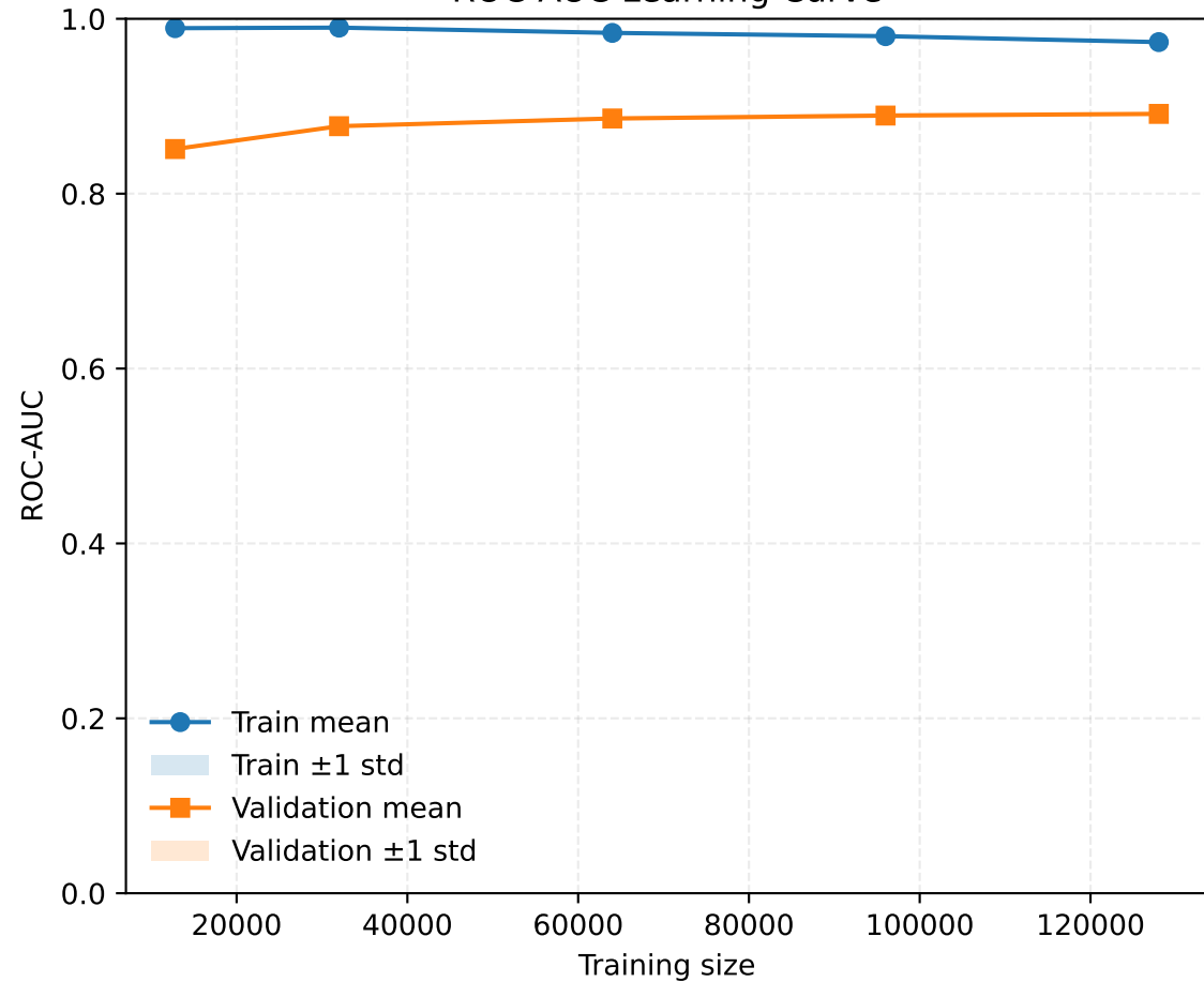
ROC-AUC Learning Curve
