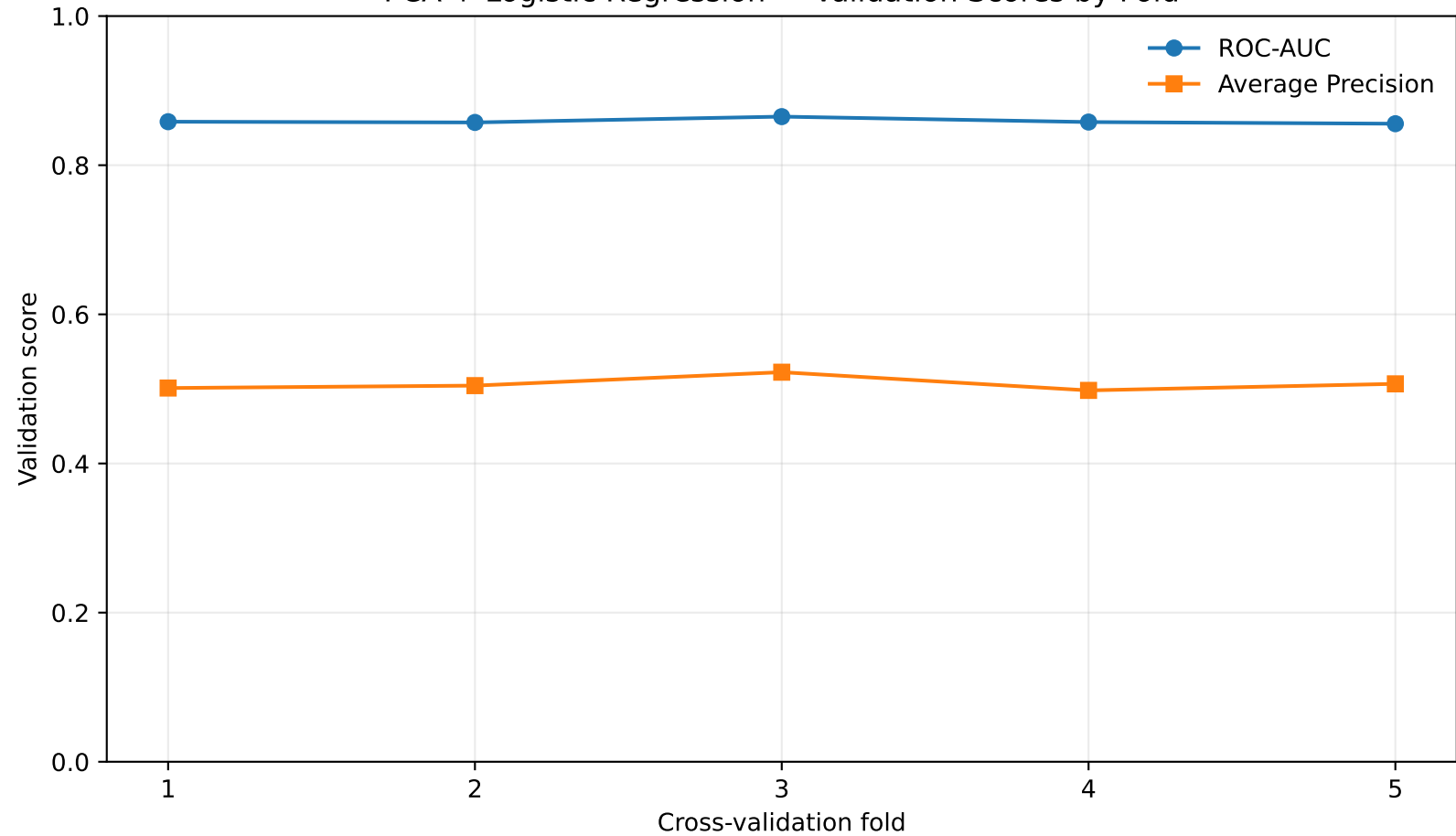
PCA + Logistic Regression — Validation Scores by Fold
