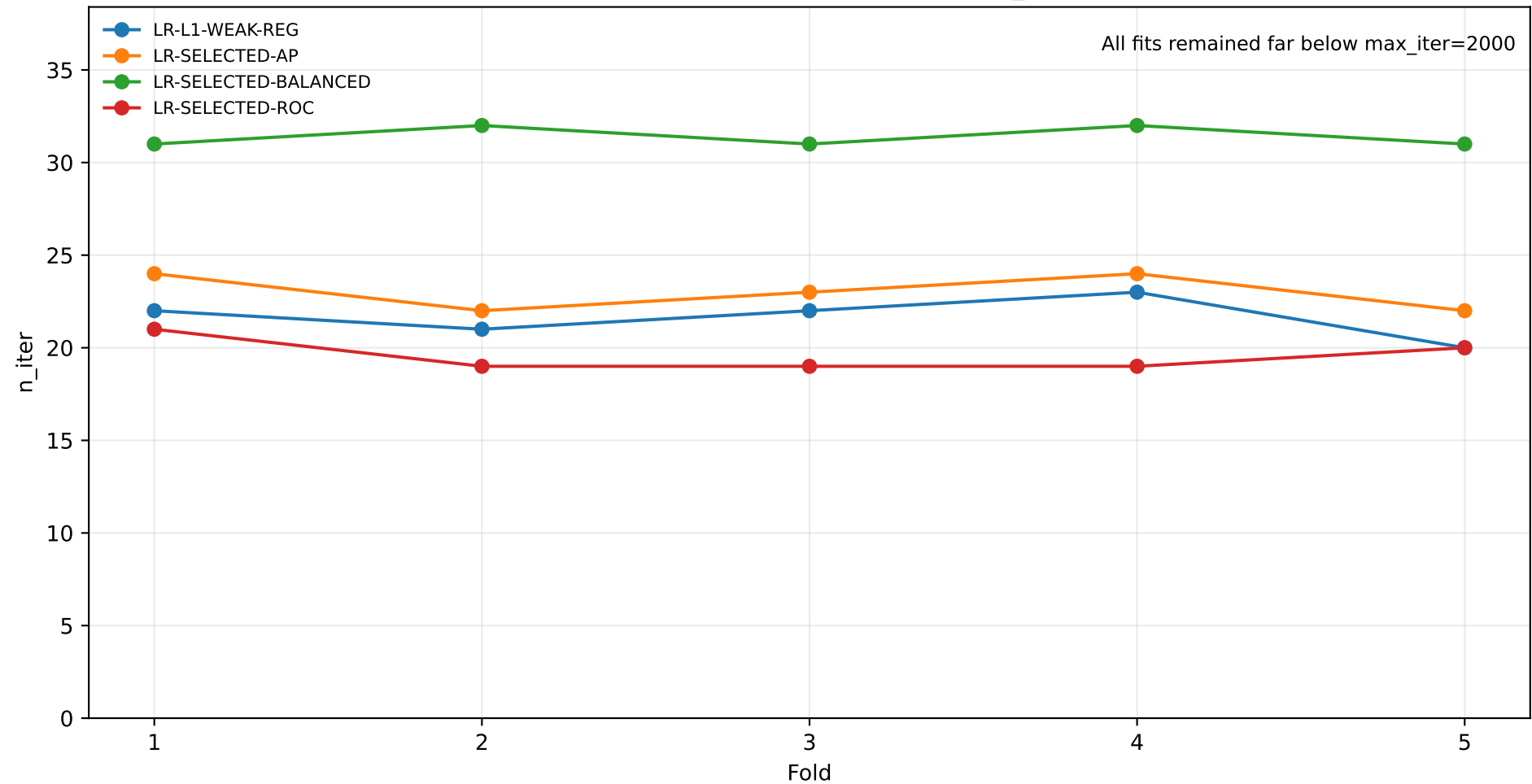
Logistic Regression Iterations by Fold (max_iter=2000)
