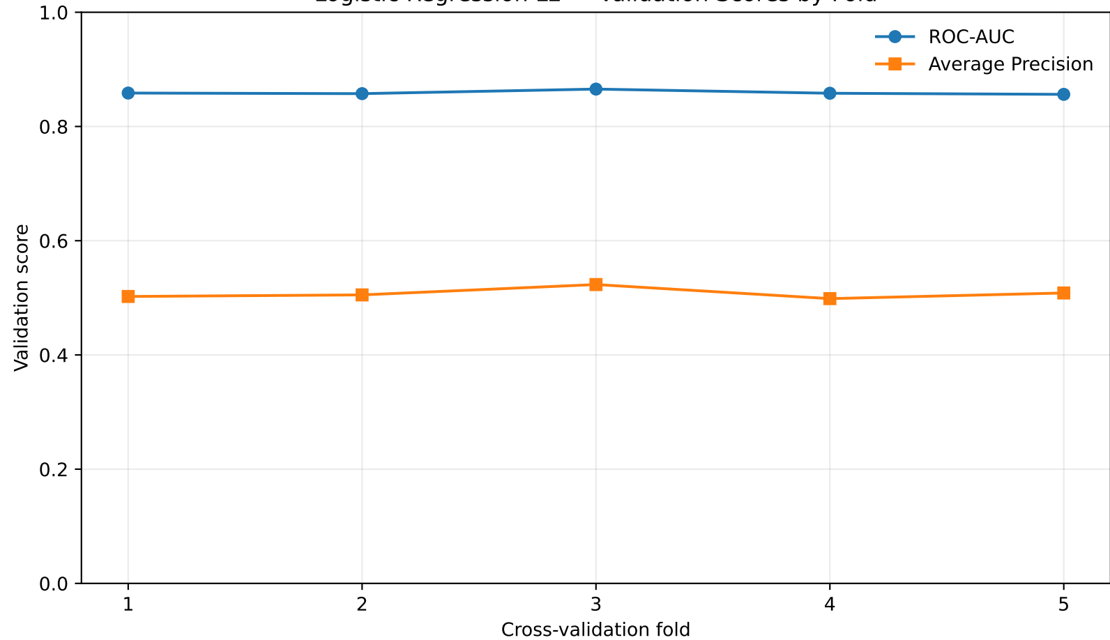
Logistic Regression L2 — Validation Scores by Fold
