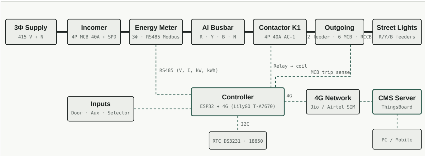
Block diagram
