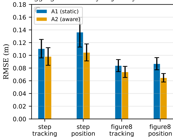
Aggregate RMSE by trajectory and metric
