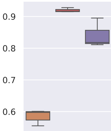
impurity
