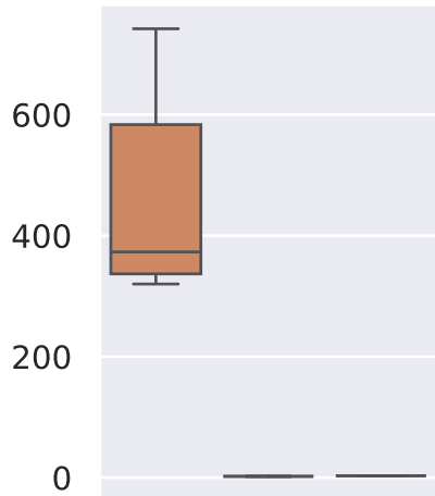
#execution contexts
