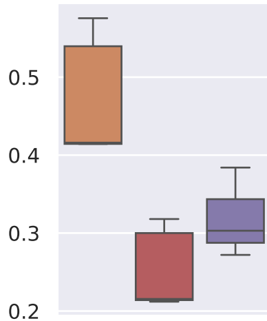
dispersal
