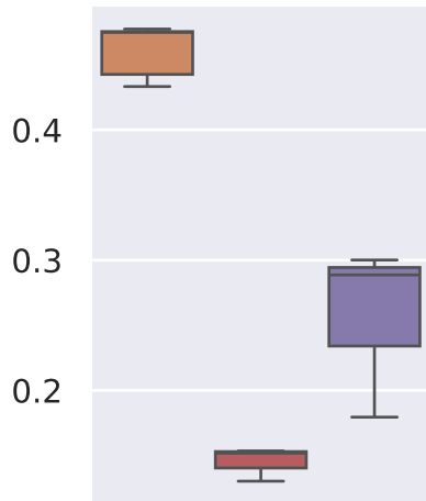
score
