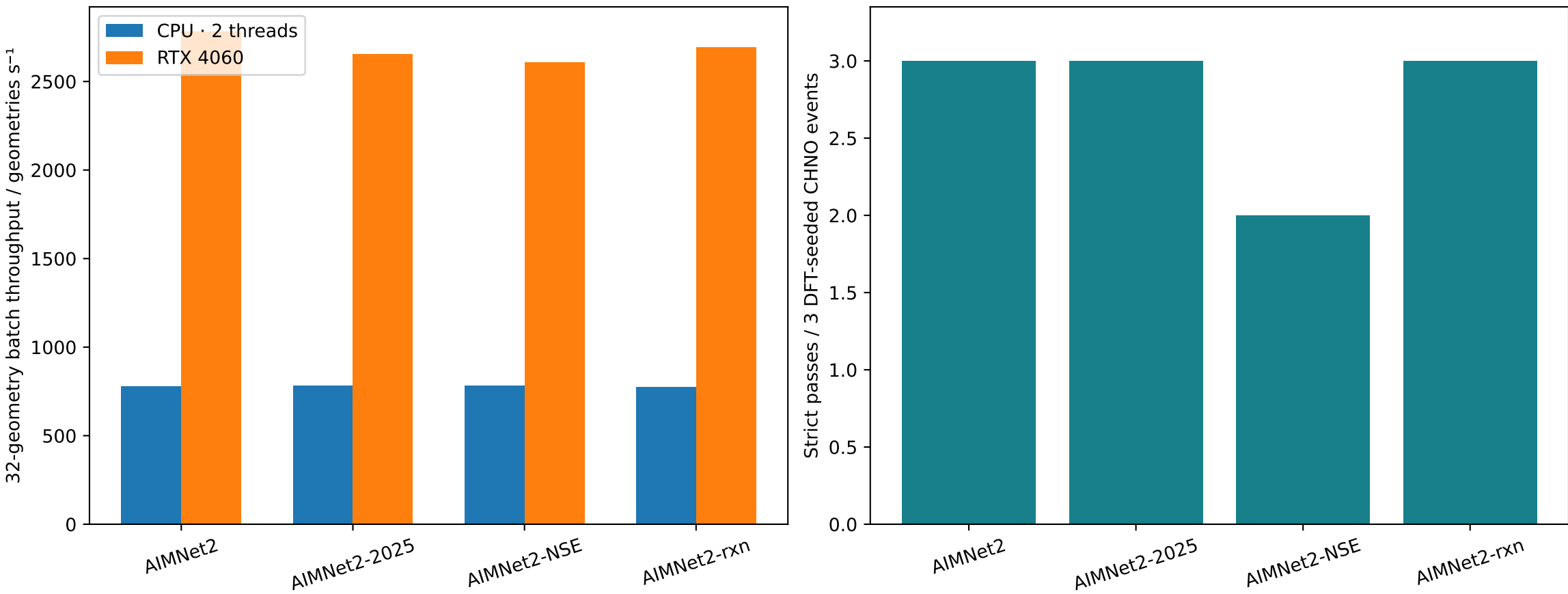
AIMNetCentral: throughput and reference-assisted reactive checks
