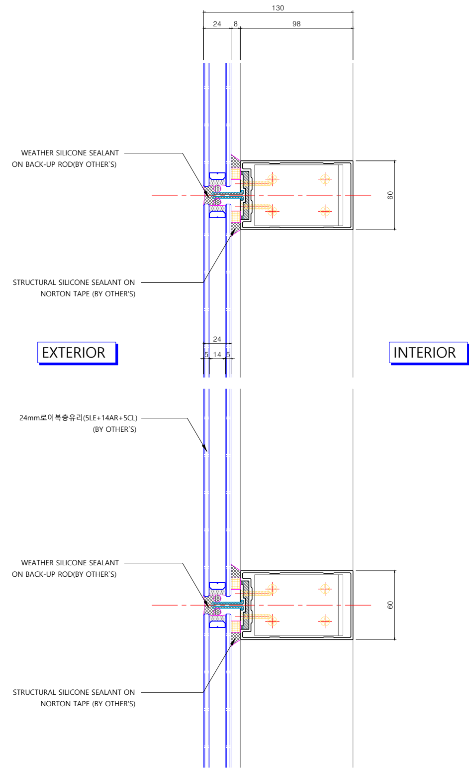
3 VERTICAL SECTION DETAIL AT 130MM SCALE : 1/3(A3)
