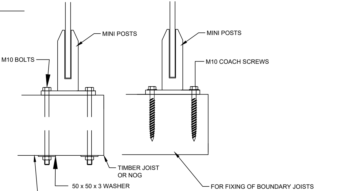
CONNECTION TO TIMBER
