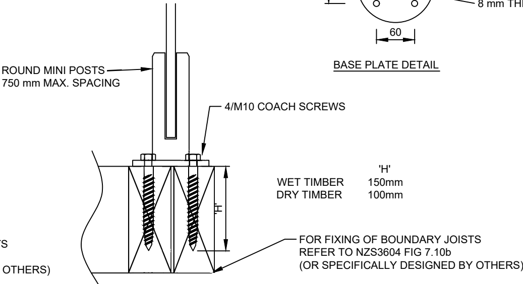
CONNECTION TO TIMBER
