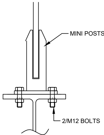
CONNECTION TO STEEL
