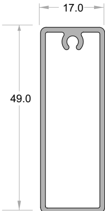
INFILL 49mm SLAT (Single Screw) JVB/030/5.35
