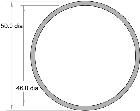
HANDRAIL JA160/5
