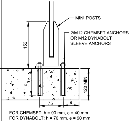
CONNECTION TO CONCRETE
