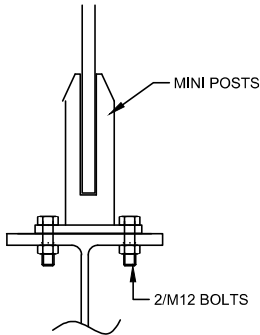
CONNECTION TO STEEL
