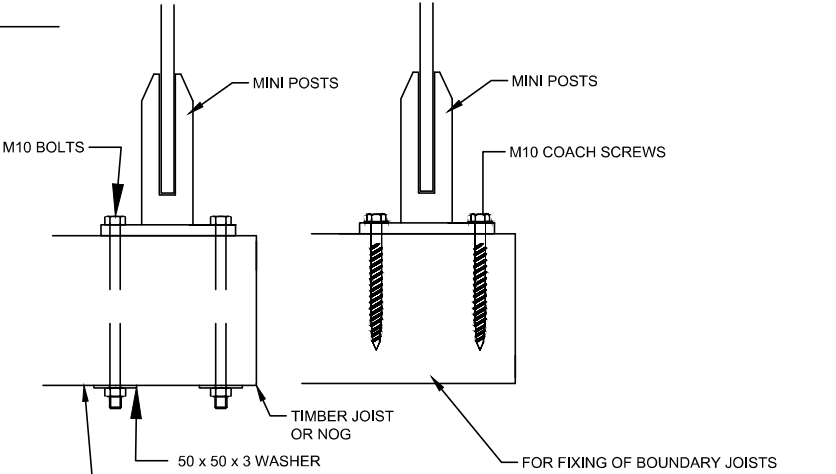
CONNECTION TO TIMBER
