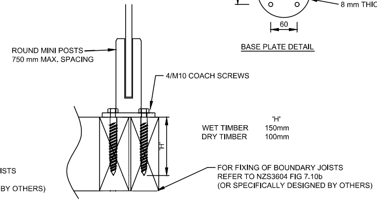
CONNECTION TO TIMBER
