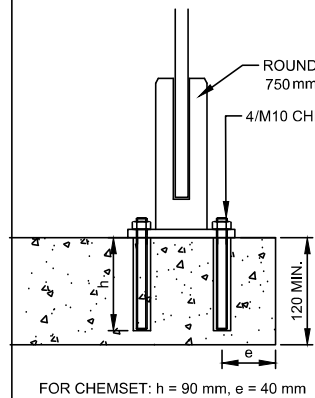
CONNECTION TO CONCRETE
