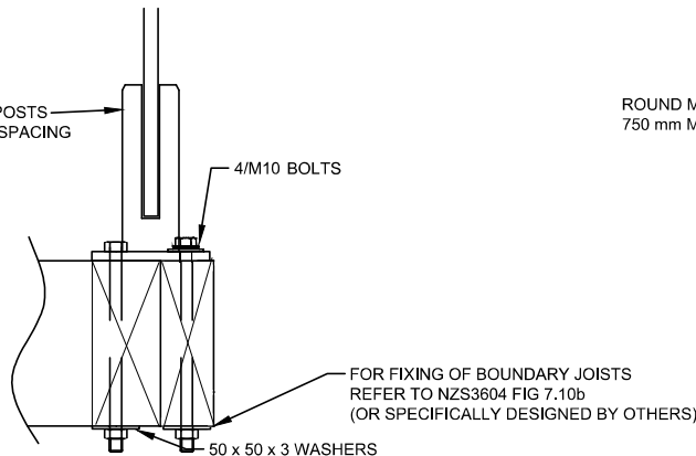
CONNECTION TO TIMBER
