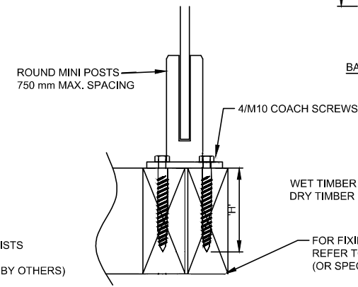
CONNECTION TO TIMBER
