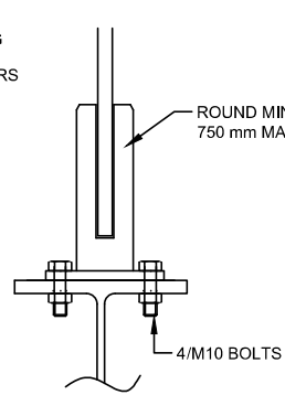
CONNECTION TO STEEL
