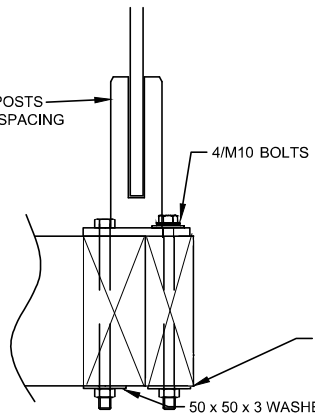
CONNECTION TO TIMBER
