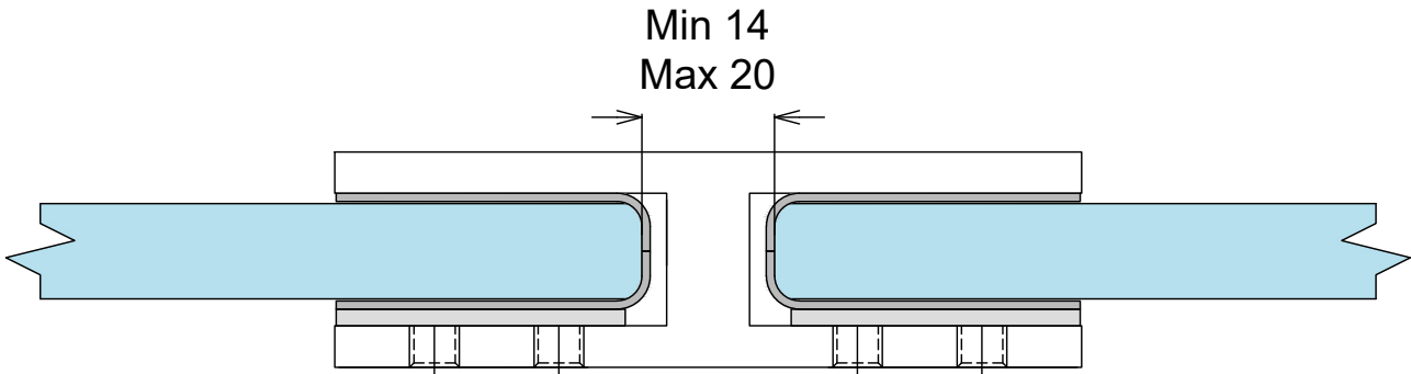
12-13.5mm GLASS - STRAIGHT CLAMP BC-180
