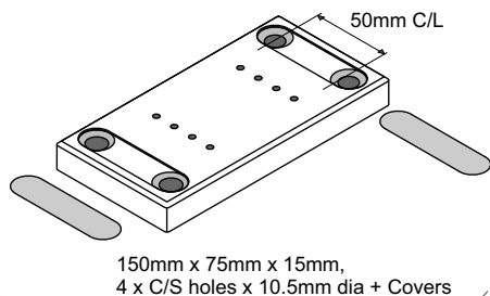
Top Cap Part No JEC 20
