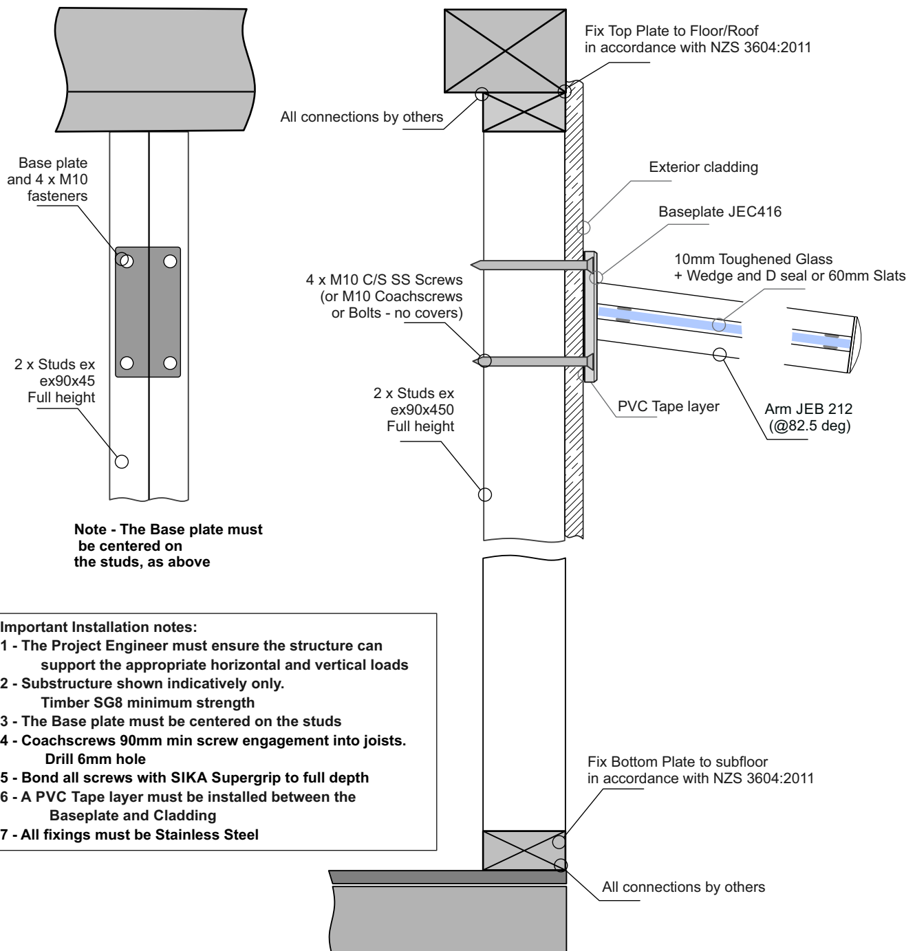
Timber Framing Wall Connection Details
