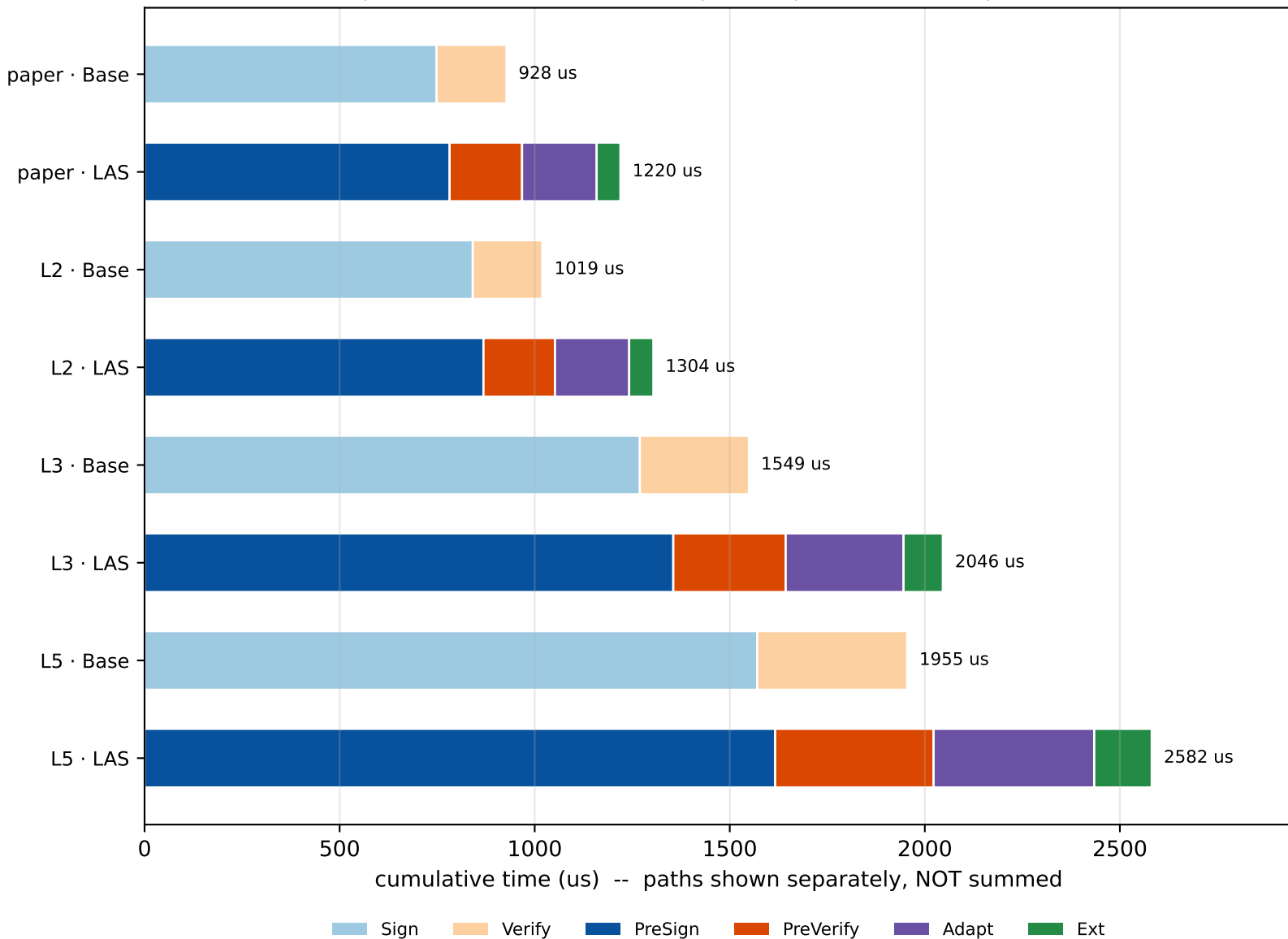
Base vs LAS protocol timelines (two separate protocols, compared not summed)
