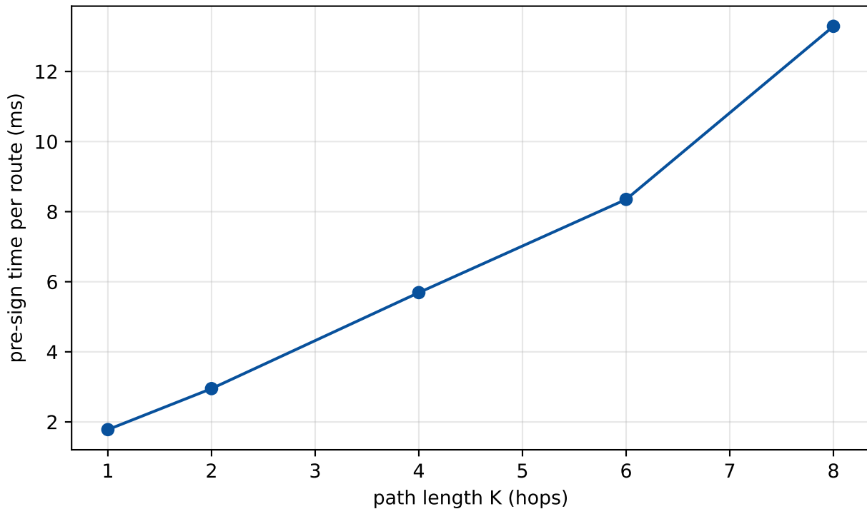
Multi-hop AMHL pre-sign time vs K (Simplified Dilithium-III)
