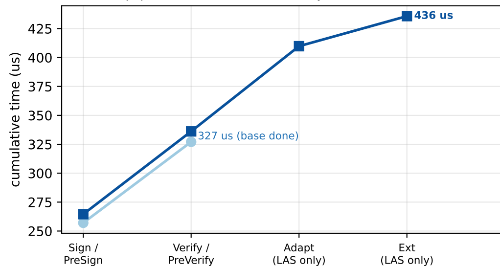
paper (n=4, ell=4) — full LAS cycle +33.2% vs base
