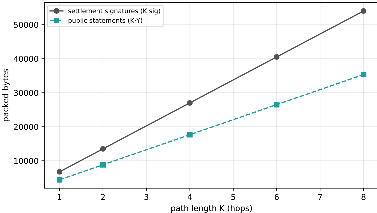
Multi-hop AMHL settlement payload vs K (Simplified Dilithium-III)
