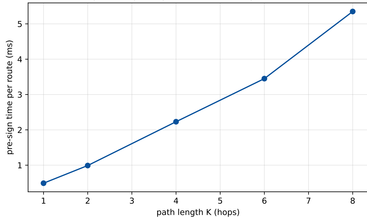
Multi-hop AMHL pre-sign time vs K (Simplified Dilithium-III)
