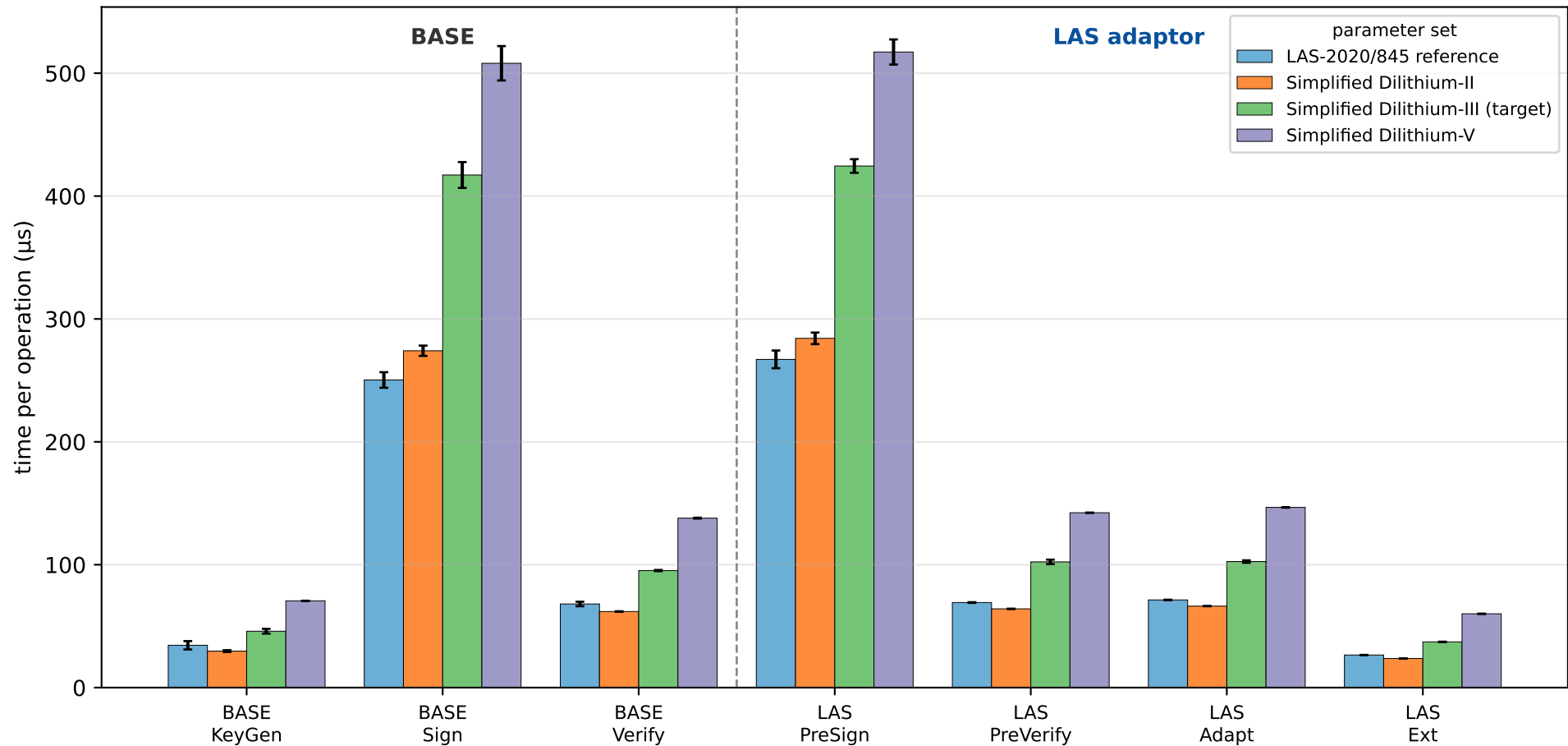
Per-operation timing ( \mu s): base signature vs LAS adaptor
