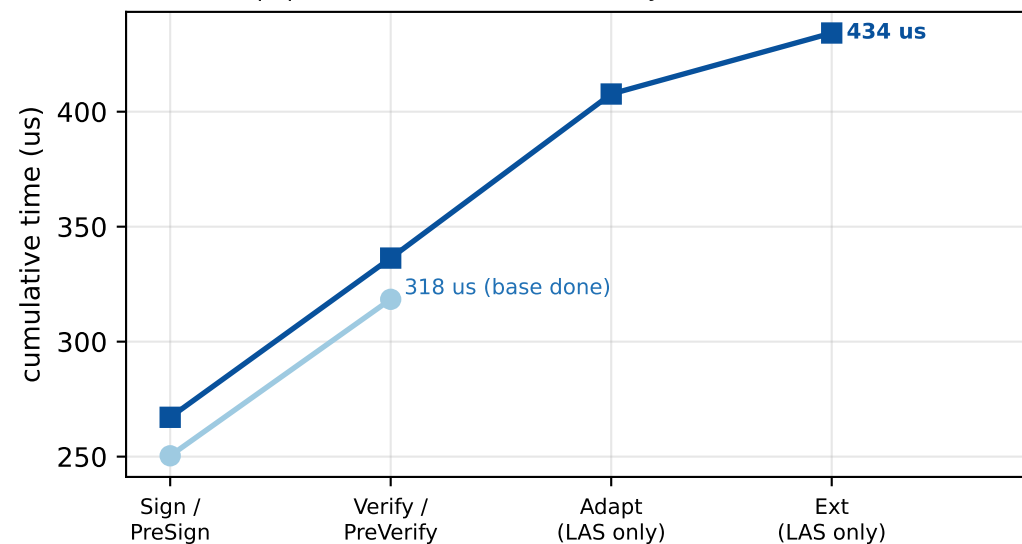
paper (n=4, ell=4) — full LAS cycle +36.4% vs base
