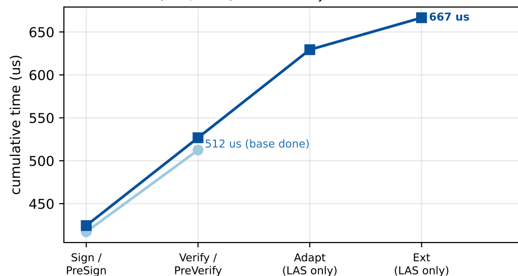
L3 (n=6, ell=5) — full LAS cycle +30.1% vs base
