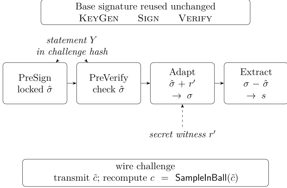
Figure 2.1: The four functions LAS adds around an unchanged base signature. PRESIGN and PREVERIFY bind the public statement Y into the challenge; ADAPT uses the witness r' to turn the pre-signature into an ordinary signature; and EXTRACT recovers a witness from that ordinary signature and the matching pre-signature. The implementation transmits \tilde{c} and re-derives c with SampleInBall .
