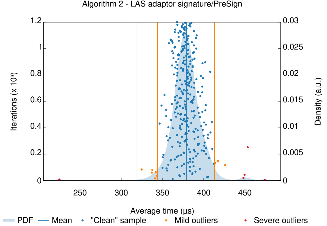
Figure 3.2: The statistical harness’s own report for PreSign at the target setting, reproduced from Criterion.rs: 300 timed samples (dots), the kernel-density estimate of the sampling distribution (shaded), the mean (vertical blue line), and Criterion’s automatic outlier classification (mild / severe, orange / red). Four presentational changes were made to Criterion’s SVG: the type enlarged, the legend moved from the right-hand column into the row beneath the plot, the margins re-flowed and cropped, and gnuplot’s three-part exponent rendered as the single glyph 10^3 . Inside the plot frame the coordinate map is the identity, so no plotted value, curve, mean, axis scale or outlier classification is altered. This is the evidence behind the Criterion column of table 3.3: a well-formed, single-mode distribution whose spread is consistent with rejection sampling and runtime noise, with 14 of the 300 samples classified as outliers (9 mild, 5 severe).
