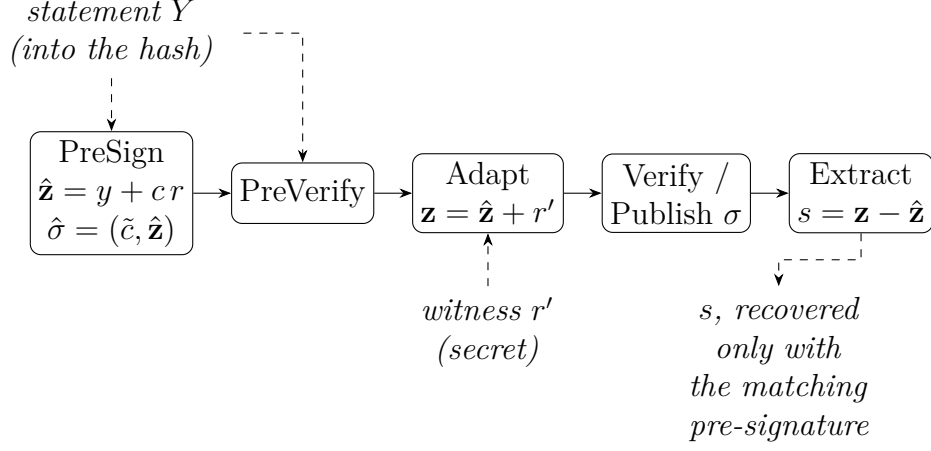
Figure 2.2: The LAS adaptor data flow, in the symbols of fig. 2.1: y is PreSign’s mask, r' the honest witness, s what Extract recovers, and c = \text{SampleInBall}(\tilde{c}) , with \tilde{c} the transmitted challenge digest. The statement Y is folded into the challenge hash during PreSign and PreVerify; the witness is added by Adapt to turn the pre-signature into a base signature; and publishing that signature lets anyone holding the pre-signature run Extract to recover it. This last step is what an atomic swap uses.
