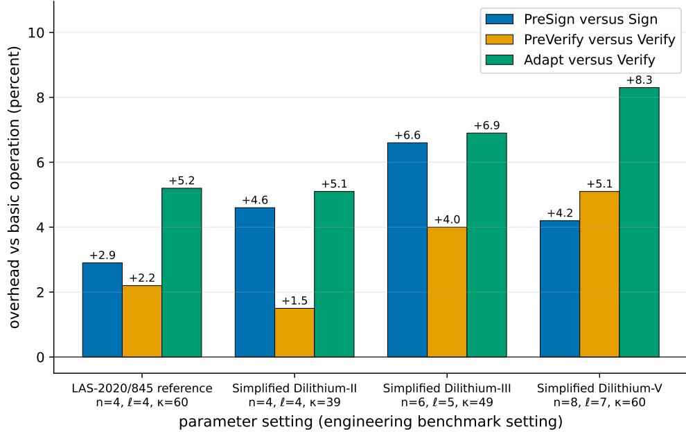
Figure A.1: Parameter sensitivity of the adaptor overhead: each LAS adaptor operation as a percentage over the basic operation it mirrors, at the four parameter sets of table 2.1. PreSign is paired with Sign; PreVerify and Adapt with Verify; Extract has no basic analogue and is omitted. The core-tier premium stays in the single digits everywhere, so adding adaptor functionality does not become more expensive as the scheme is scaled up. This is a secondary robustness check; the primary comparison is the per-operation overhead at the target setting, table 3.2.
