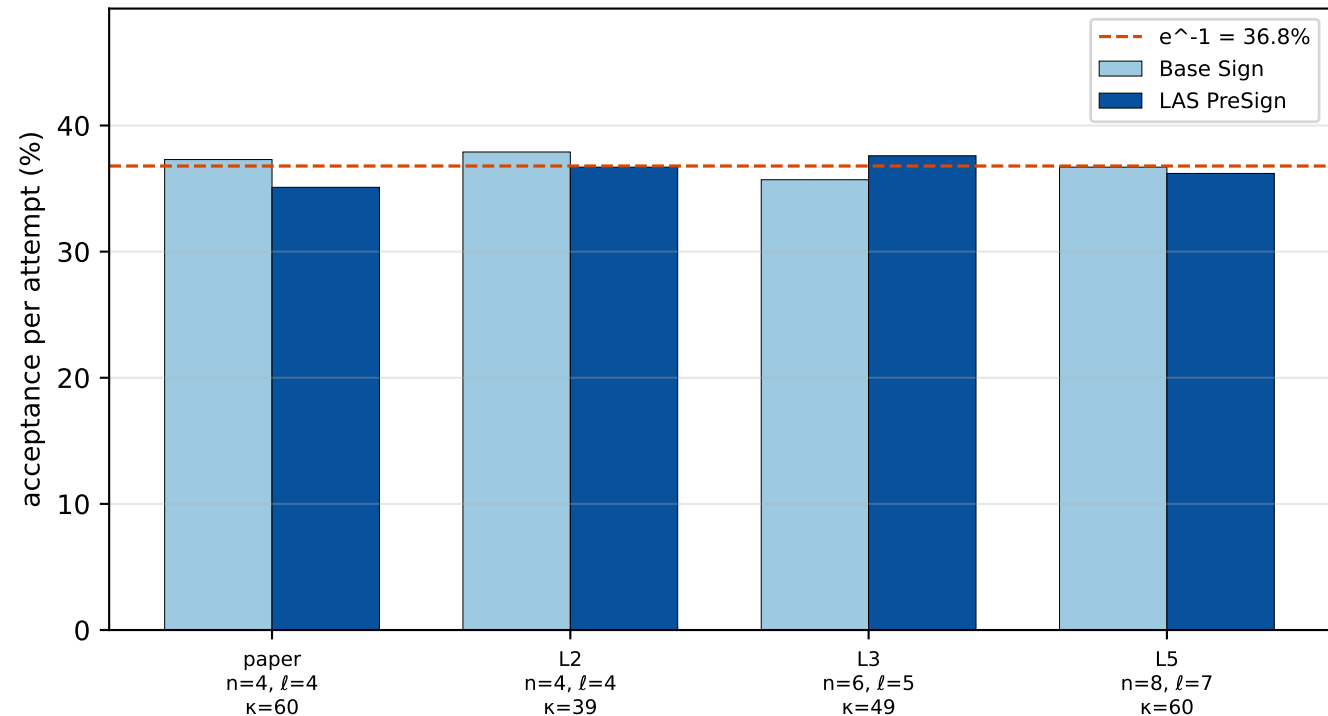
Rejection sampling is stable across parameter sets ( \sim 37\% , \sim e^{-1} )
