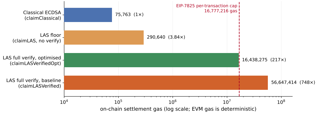
Figure 3.7: The claim paths of table 3.7 on a logarithmic axis, which is what makes the spread legible. The dashed line is the EIP-7825 cap on the transaction gas limit ( 16\,777\,216 = 2^{24} ): the baseline verifier’s bar crosses it, while the restructured claimLASVerifiedOpt — same scheme, same predicate under the registration invariant of table 3.7, different expression — falls below. All four bars come from one -gas-report table and so are mutually comparable; the under-the-cap claim itself rests on the separate real-client run described in table 3.7.
