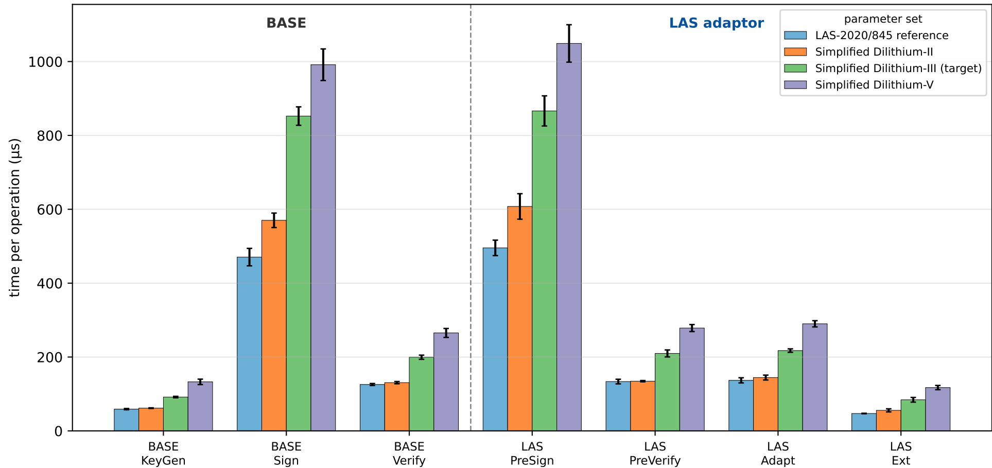
Per-operation timing ( \mu\text{s} ): base signature vs LAS adaptor
