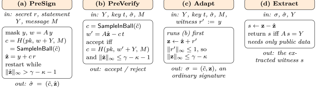
Figure 2.1: The four functions LAS adds to the base signature, one panel each: what goes in, what the function computes, and what comes out. KEYGEN, SIGN and VERIFY are reused unchanged and are not shown. Two asymmetries are the whole construction. Only (a) and (b) fold the statement Y into the challenge hash — which is why the adaptor layer inherits the base scheme’s arithmetic rather than replacing it, (d) using Y only to check the recovered witness; only (c) and (d) touch the witness, and they are the two functions a basic signature has no counterpart for. Each panel’s arithmetic is that of Algorithm 2 of [10], including its symbols: y is the mask PRESIGN samples, so the response it returns is \hat{z} = y + cr under the secret r ; the witness of the pair (Y, y) is written r' from the point where it enters the arithmetic, as that algorithm’s ADAPT step parses it; and EXTRACT returns s , which is r' on an honest run but in general only a witness of the extended relation (table 2.2). How the four compose, and why publishing \sigma is what makes a swap atomic, is fig. 2.2.
