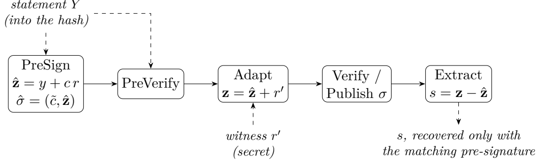
Figure 2.2: The LAS adaptor data flow, in the symbols of fig. 2.1: y is PreSign’s mask, r' the honest witness, s what Extract recovers. The statement Y is folded into the challenge hash during PreSign and PreVerify; the witness is added by Adapt to turn the pre-signature into a base signature; and publishing that signature lets anyone holding the pre-signature run Extract to recover it. This last step is what makes an atomic swap atomic.
