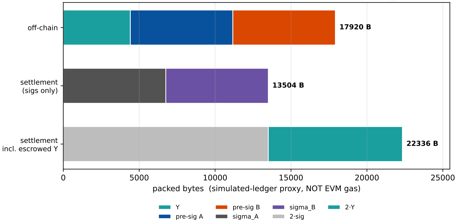
Atomic-swap payload breakdown (Simplified Dilithium-III; bench_app3)
