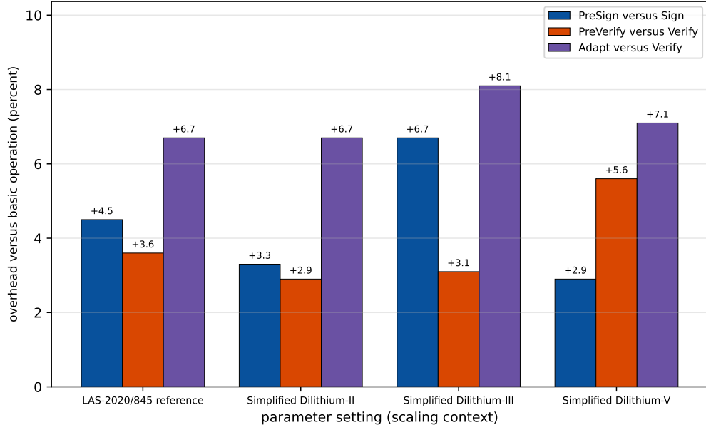
Figure A.1: Parameter sensitivity of the adaptor overhead: each LAS adaptor operation as a percentage over the basic operation it mirrors, at the four parameter sets of table 2.2. PreSign is paired with Sign; PreVerify and Adapt with Verify; Extract has no basic analogue and is omitted. The premium stays in the single digits everywhere, so adding adaptor functionality does not become more expensive as the scheme is scaled up. This is a secondary robustness check; the primary comparison is the per-operation overhead at the target setting, table A.2.
