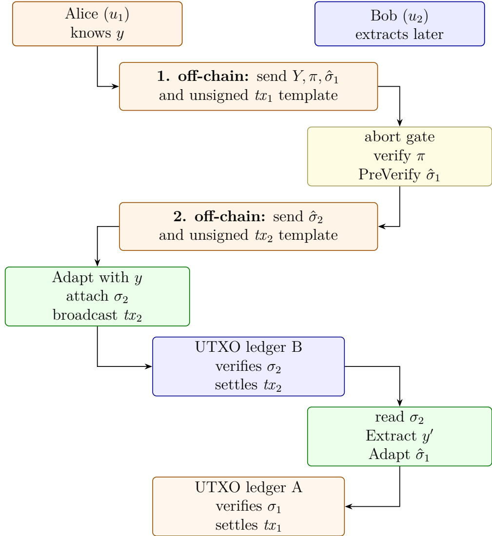
Figure 2.4: The atomic-swap protocol used in the UTXO study, adapted from Figure 1 of [10]. Only the two adapted signatures reach ledgers, inside the ordinary signature/witness field of their own transactions; Y, \pi , the unsigned templates and the pre-signatures are off-chain protocol messages, and the witness y is never transmitted. Step 1 gives Bob enough evidence to decide whether to continue; step 2 gives Alice the pre-signature she can adapt with y ; once \sigma_2 is visible in the settled transaction on ledger B, Bob extracts y' and adapts the first leg for ledger A. The signed message m_i is the signature hash of the unsigned template tx_i , not the transaction bytes themselves. Section 3.6 reports the assertions that this flow passed, and section 3.7 measures its cost.
