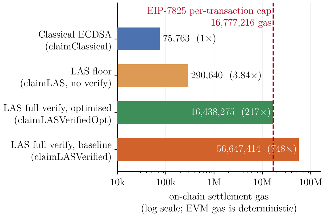
Figure 3.6: The claim paths of table 3.10 on a logarithmic axis, which is what makes the spread legible. The dashed line is the EIP-7825 cap on the transaction gas limit ( 16\,777\,216 = 2^{24} ): the baseline verifier’s bar crosses it, while the restructured claimLASVerifiedOpt — same scheme, same predicate under the registration invariant of table 3.10, different expression — falls below. All four bars come from one -gas-report table and so are mutually comparable; the under-the-cap claim itself rests on the separate real-client run described in table 3.10.
