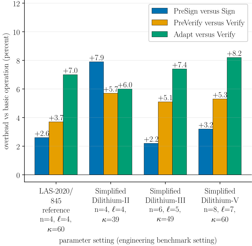
Figure 3.2: Parameter sensitivity of the adaptor overhead: each LAS adaptor operation as a percentage over the basic operation it mirrors, at the four parameter sets of table 2.1. PreSign is paired with Sign; PreVerify and Adapt with Verify; Extract has no basic analogue and is omitted. The core-tier premium remains small across the sweep: all target-setting adaptor operations are single-digit, and the maximum over all parameter sets is +8.2%. This is a secondary robustness check on the headline of fig. 3.1, not a result about scaling: the primary comparison is the per-operation overhead at the target setting, table 3.2. The absolute timings behind every bar are table A.5 (appendix).
