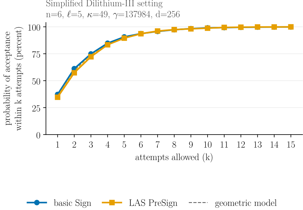
Figure 3.3: The probability that a sign-class call has been accepted within k rejection-sampling attempts, at the target setting Simplified Dilithium-III . The solid curves are measured: the empirical distribution of the same 2000-call sample table 3.3 summarises, counted per attempt on the C implementation — basic Sign (blue) under the bound \gamma - \kappa , LAS PreSign (orange) under the tighter \gamma - \kappa - 1 . The dashed lines are the closed-form geometric model of eq. (2.2) for those two bounds, predicting first-attempt acceptance of 36.8% and 36.0% respectively; measurement and model are drawn together so their agreement can be read off rather than asserted. The two measured curves are nearly coincident, which is exactly why the PreSign-versus-Sign timing gap is so small. Both pass 90% within six attempts — five clears it for Sign but not for PreSign, whose bound is the tighter of the two — and then flatten. That flattening is the practical point: allowing many more attempts buys almost nothing, because the overwhelming majority of calls are accepted within the first few.
