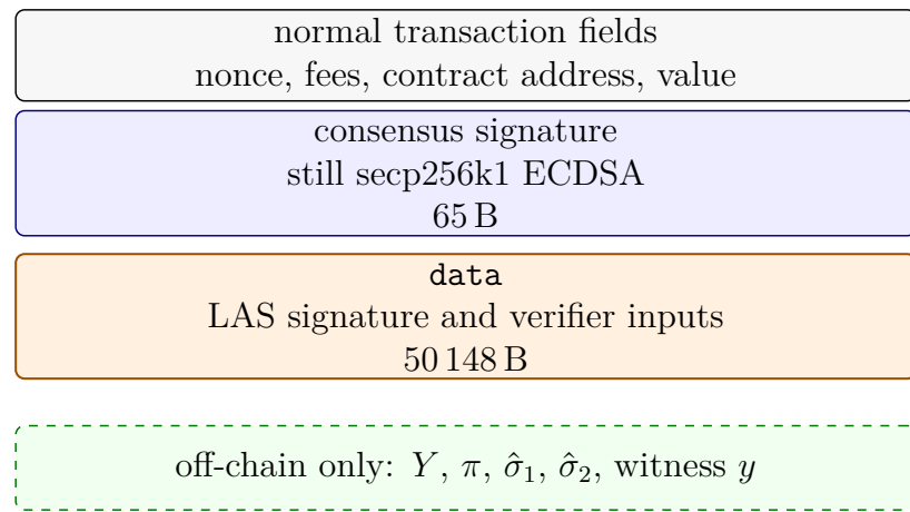
Figure 3.7: The same settlement on Ethereum: the claim transaction of the client run in table 3.10, read against the UTXO counterpart in fig. 3.5. Neither venue gains a field from the adaptor layer, but the lattice signature lands in a different structural position. On a Bitcoin-like UTXO chain it must occupy the signature slot consensus checks, so the chain needs a new consensus rule before it can verify LAS. On the EVM the authorising transaction signature remains secp256k1; the lattice signature rides in data as an argument to a contract. Contracts therefore make Ethereum the more flexible venue and Bitcoin the more restricted one here. The 50 148 B is measured from the client receipt and is the whole calldata payload, not the signature alone.
