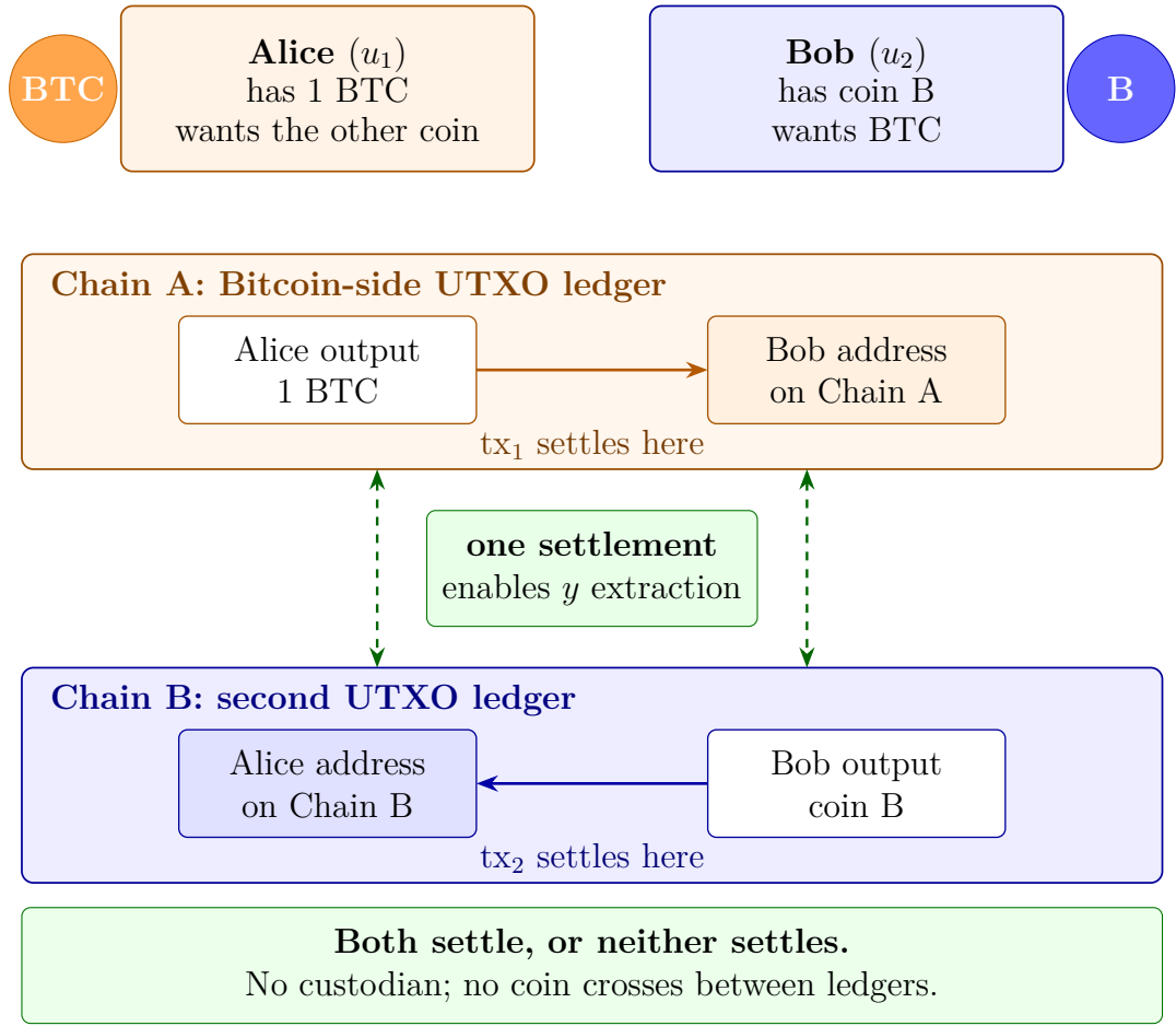
Figure 1.2: A motivation-level picture of an atomic swap, one concrete blockchain application of adaptor signatures. Alice and Bob trade assets recorded on two different ledgers. Each payment is an ordinary transaction on its own chain: tx_1 moves Alice’s Chain-A coin to an address Bob owns, while tx_2 moves Bob’s Chain-B coin to an address Alice owns. No coin crosses chains; the cross-chain object is the secret witness, which the counterparty extracts from the published signature using its matching pre-signature. Adaptor signatures provide this cryptographic link without requiring the swap condition to appear as a separate on-chain script. The two parties are named as in Esgin et al. [10], whose u_1 and u_2 the later chapters use; fig. 2.4 sets the exchange out message by message.
