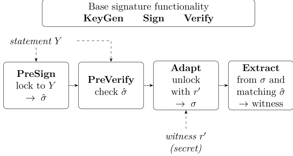
Figure 2.1: What changes when a base signature becomes an adaptor signature. Base SIGN and VERIFY remain the signature interface; LAS adds PRESIGN and PREVERIFY, which lock signing to the public statement Y , ADAPT, which unlocks a pre-signature \hat{\sigma} using the secret witness r' to give an ordinary signature \sigma , and EXTRACT, which recovers a witness from \sigma together with its matching pre-signature. GEN produces (Y, r') from the same key-generation relation. Extraction needing both objects is why publishing \sigma reveals the witness only to a party already holding \hat{\sigma} , which is the step an atomic swap uses. The algebra of each operation follows in the text.
