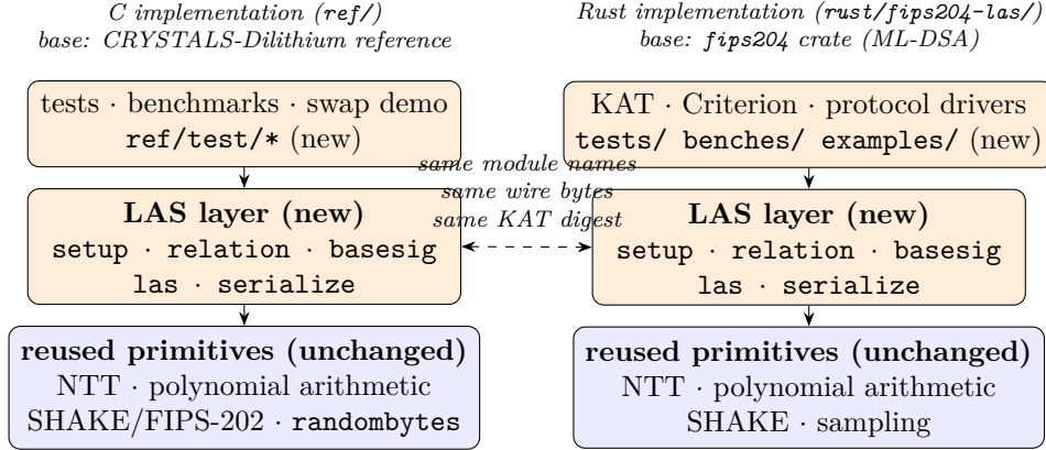
Figure 2.2: Repository structure. Both implementations have the same shape: a new, self-contained LAS layer (orange) — the same five modules under the same names — built on an unmodified base of reused lattice primitives (blue), with the tests and benchmarks on top. The two columns are tied together by construction: identical wire bytes and the shared pinned known-answer digest (bb6ad0da...260c). This is the high-level map for reading the code; the per-file classification is table 2.1.
