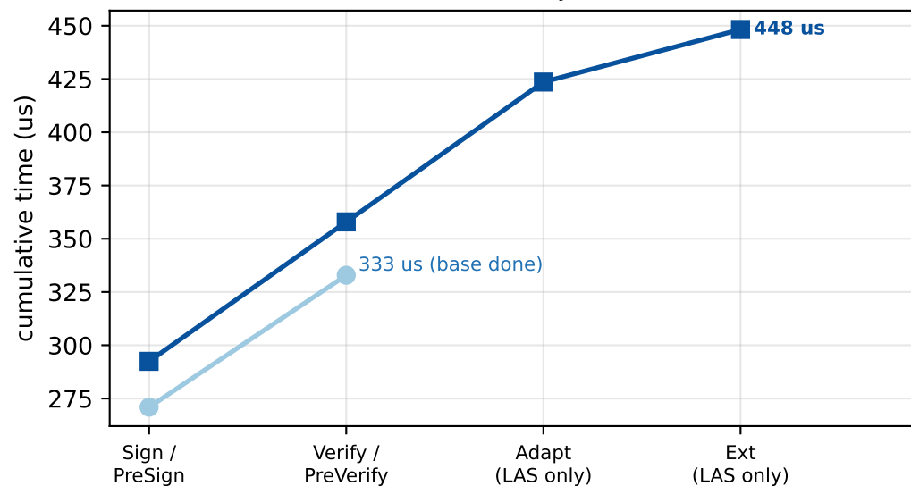
L2 (n=4, ell=4) — full LAS cycle +34.7% vs base
