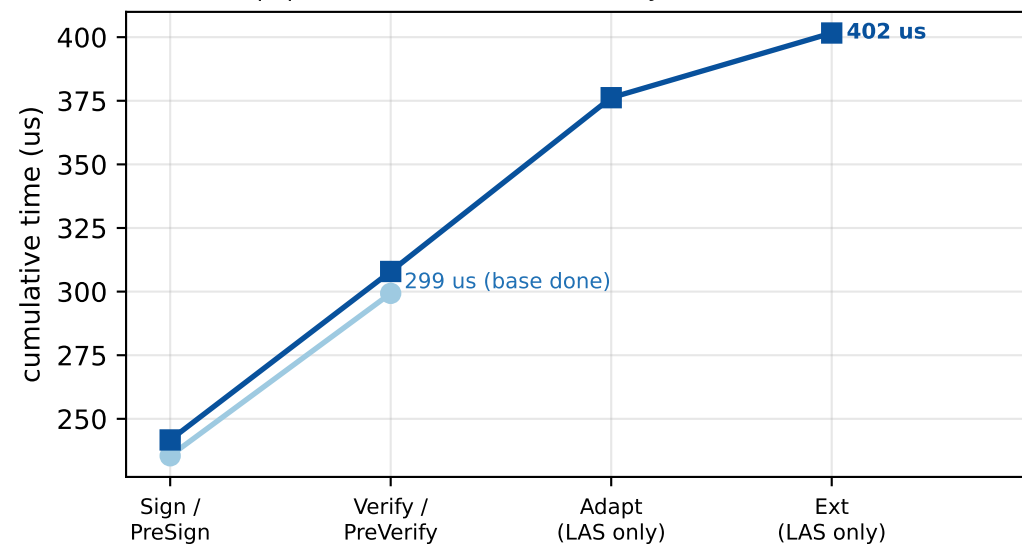
paper (n=4, ell=4) — full LAS cycle +34.2% vs base
