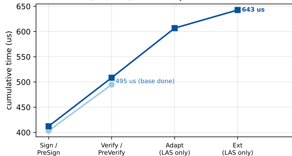
L3 (n=6, ell=5) — full LAS cycle +29.9% vs base
