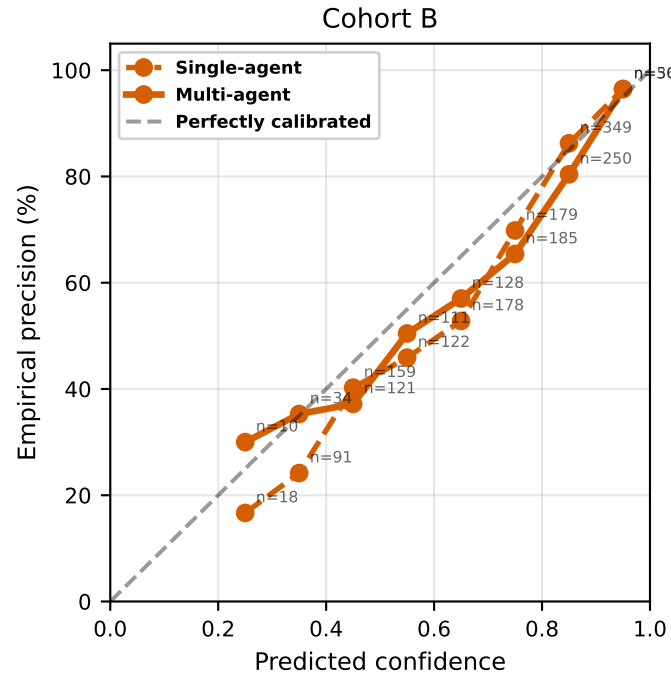
Reliability Diagram
