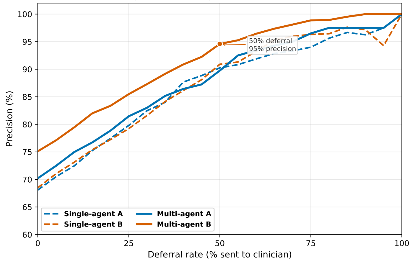
Deferral Rate vs Precision (Single- and Multi-Agent BMA Beta-Binomial)
