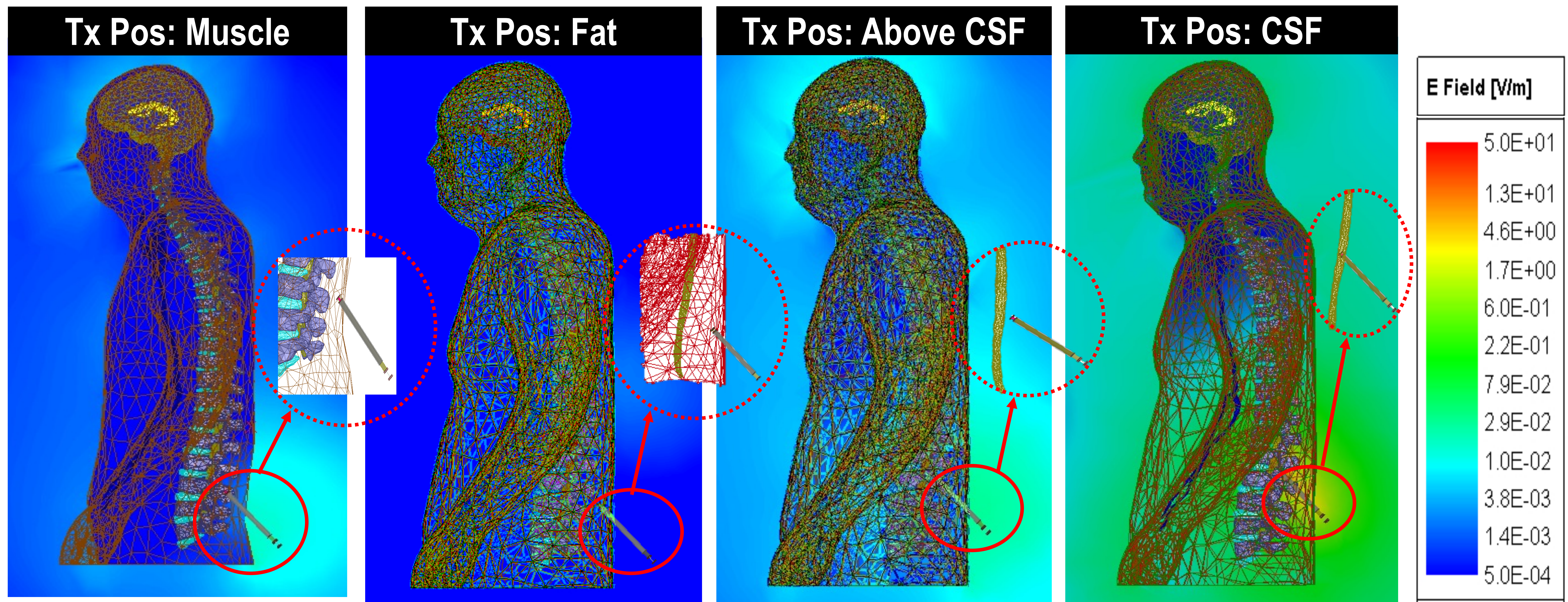
(A) E-Field Plots in Simplified Neva Model
