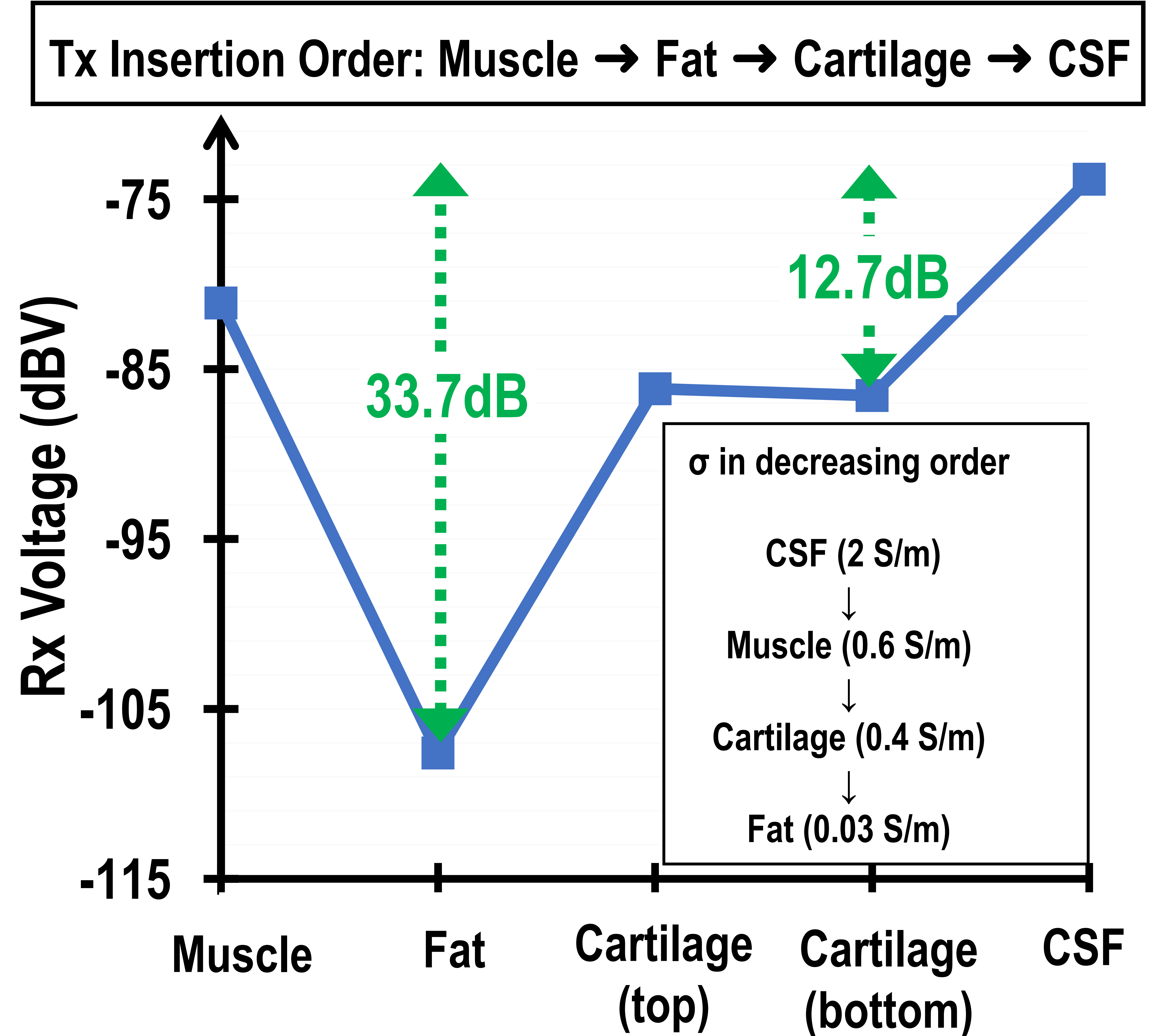
(C) Received Voltage from each layer
