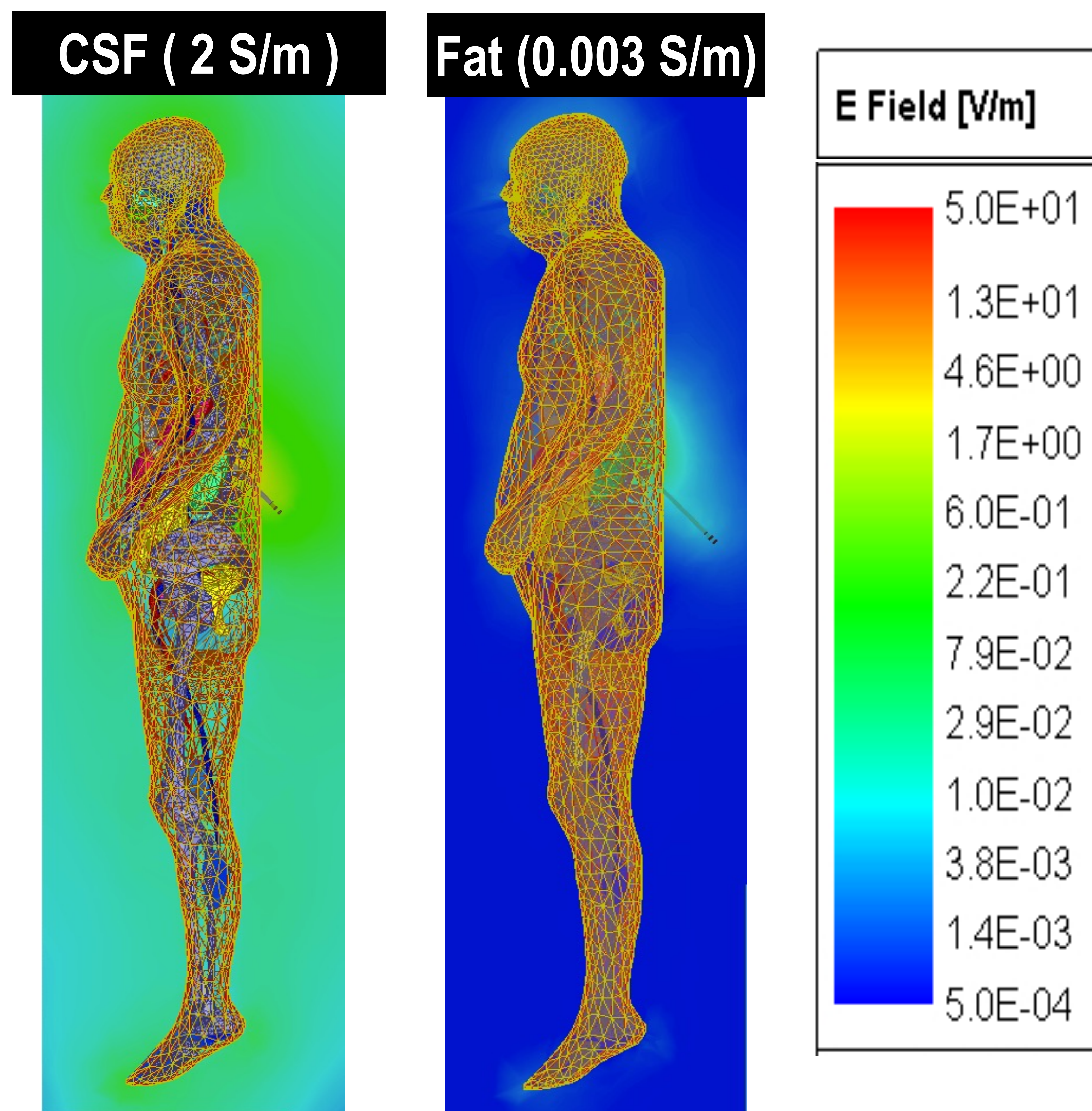
(B) E-Field Plots in Full Neva Model
