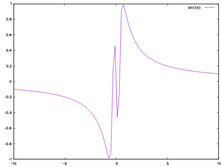
Figure 1: \sin\left(\frac{1}{x}\right)
