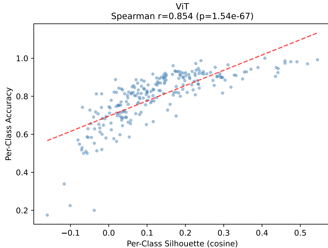
Per-Class Silhouette vs Accuracy
